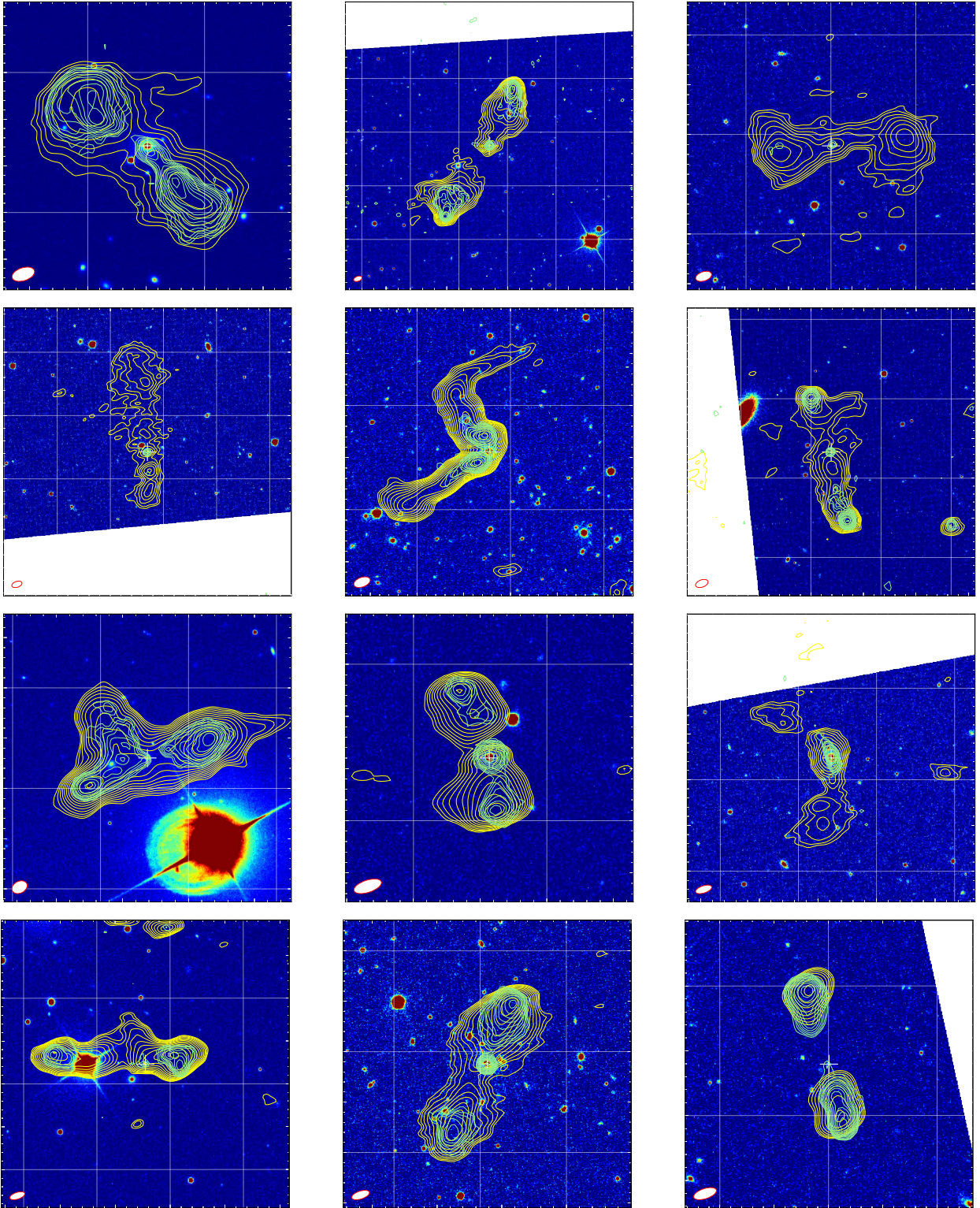
Figure B2. Postage stamps of example sources with FIRST cores. Colours, contours and lines as in Fig. A1. From left to right, top to bottom: SDSS J124541.96+332428.5, J125541.50+250744.7, J125715.99+312153.1, J130057.21+325625.5, J130856.91+261333.2, J131246.85+275219.8, J132713.87+285318.1, J133449.73+312824.0, J133738.33+312514.2, J133837.35+311413.8, J134251.68+311052.6, and J134747.98+325823.8.
