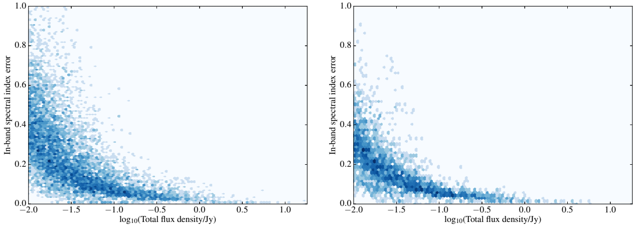
Figure 8. Density plot of errors on the in-band spectral index as a function of total LOFAR flux density. Left: all sources and fields. Right: only the central 2 degrees of the NW, NE and SW fields are plotted.
