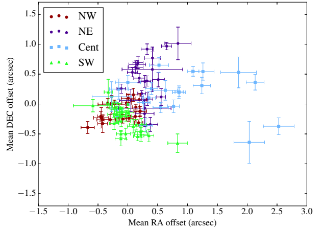
Figure 6. FIRST/LOFAR offsets in the field. The mean offset for each facet is plotted individually. Error bars show the nominal errors on the mean offsets.
