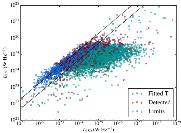
Figure 15. 250- \mu\text{m} far-infrared luminosity, estimated as described in the text, as a function of LOFAR radio luminosity. Objects are colour coded depending on whether they have temperature measurements, are detected at the 2\sigma level at 250 \mu\text{m} but without a valid temperature measurement, or are 2\sigma upper limits at 250 \mu\text{m} . The division into detected and non-detected sources at this level is for plotting purposes only and plays no part in the analysis. Solid lines show q'_{250} = 20 and q'_{250} = 5 , where q'_{250} is as defined in the text.
