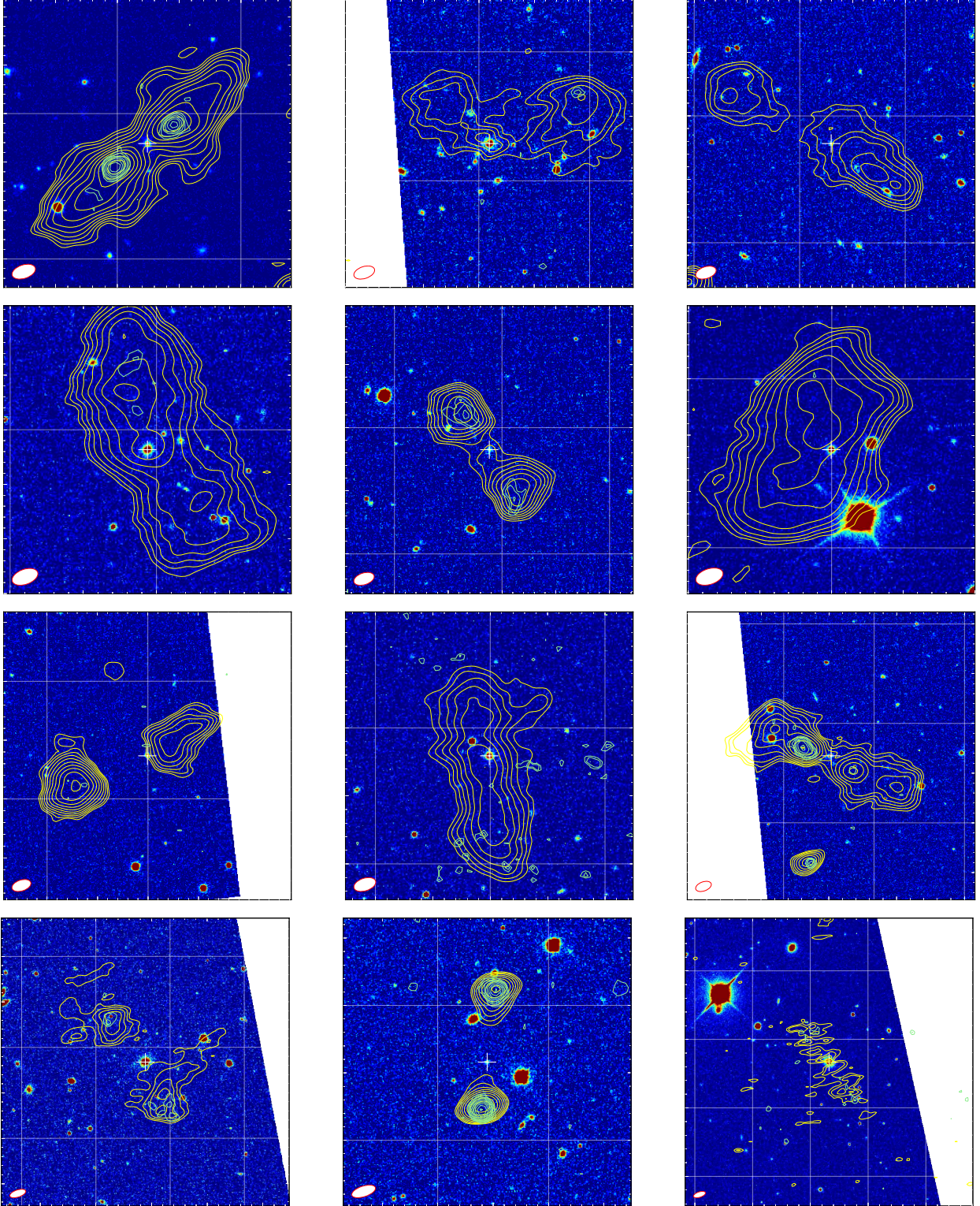
Figure B1. Postage stamps of example candidate remnant sources. Colours, contours and lines as in Fig. A1. From left to right, top to bottom: SDSS J125147.03+314047.6, J125311.62+304017.3, J125930.81+333646.9, J130004.25+263652.7, J130332.47+312949.5, J130532.02+315634.8, J130916.02+305121.9, J131040.03+322047.6, J131405.90+243240.3, J133057.34+351650.2, J133422.21+343634.8, and J134802.70+322940.1.
