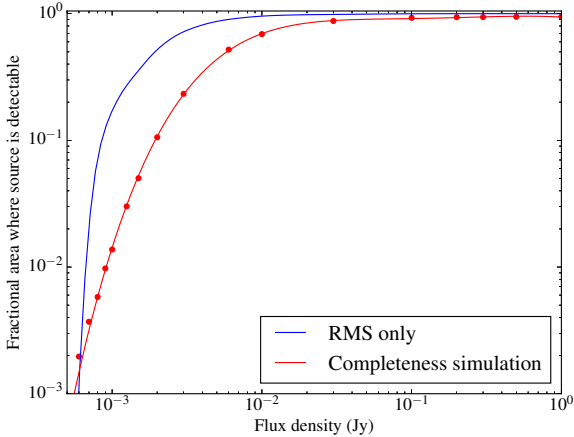
Figure 3. Completeness function for the whole survey compared with the expectations from the rms map alone. The points are the results of simulations (Poisson errors, though present, are generally smaller than symbols and are not plotted) while the smooth curve shows the best-fitting 5th-order polynomial in log space used to approximate the completeness curve and interpolate to un-simulated flux densities.
