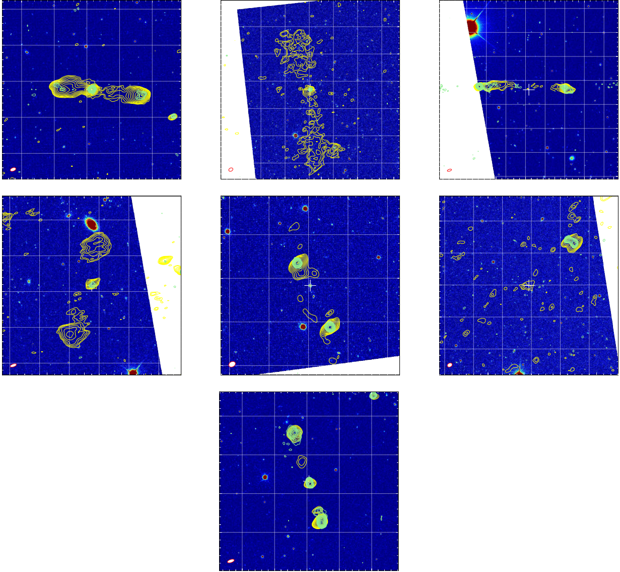
Figure A1. ‘Postage stamp’ images of the 7 optically identified objects at or close to 1 Mpc in physical size in the sample. Colours show SDSS r -band images; contours are LOFAR (yellow) and FIRST (green) contours starting at the local 3\sigma value and increasing by steps of a factor 2. An ellipse in the bottom left-hand corner shows the LOFAR beam and a white cross the location of the optical identification. Grid lines are spaced by 1 arcmin in right ascension and declination: north is up. Top row, from left to right, are: SDSS J133127.82+250050.0 ( z = 0.8040 , D = 0.9 Mpc), J134415.75+331719.1 ( z = 0.6863 , D = 1.0 Mpc), and J130451.41+245445.9 ( z = 0.6025 , D = 1.0 Mpc). Middle row: J132928.99+333810.1 ( z = 0.5404 , D = 1.0 Mpc), and J132735.32+350636.7 ( z = 0.5003 , D = 1.4 Mpc), J133744.35+251359.0 ( z = 0.6816 , D = 1.2 Mpc). Bottom: J131443.83+273741.3 ( z = 0.4179 , D = 1.1 Mpc).
