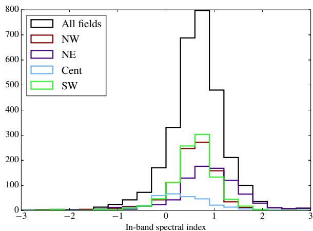
Figure 7. In-band spectral index determined from LOFAR data. The overall histogram is shown together with the histograms for each field.
