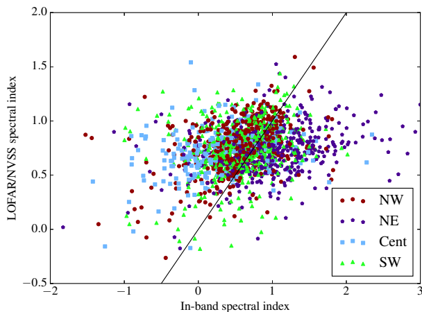
Figure 10. The in-band and NVSS/LOFAR spectral indices compared. The solid line shows equality between the two spectral indices. In general increasing spectral steepness with frequency means that we would expect points to lie above this line.
