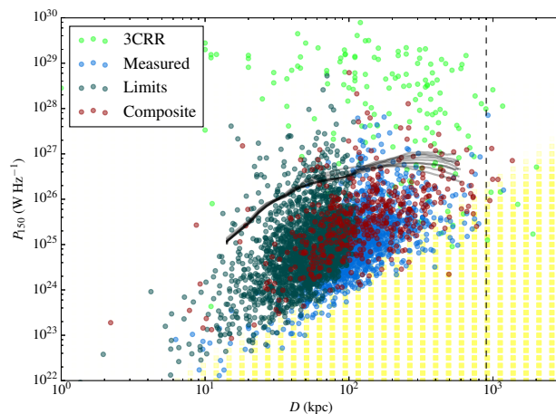
Figure 18. The power/linear-size diagram for AGN in our survey and for 3CRR objects. For the LOFAR AGN, we plot separately sources with angular sizes smaller than 15 arcsec as measured by PYBDSM, where the physical sizes should probably be considered upper limits; sources with larger sizes, probably at least somewhat meaningfully measured by PYBDSM; and composite sources, whose largest component separation is used as a proxy for their size. 3CRR sizes are all measured from high-resolution radio maps. Boxes indicate the region where some or all LOFAR sources in the range z = 0 to z = 0.8 with uniform surface brightness would drop below the detection threshold for our images. The vertical dashed line indicates our giant-radio-galaxy selection criterion (see the text for details). The grey curves represent tracks in the diagram for a source with a jet power of 10^{38} W, in various environments, derived from the modelling of Hardcastle & Krause (2014) .
