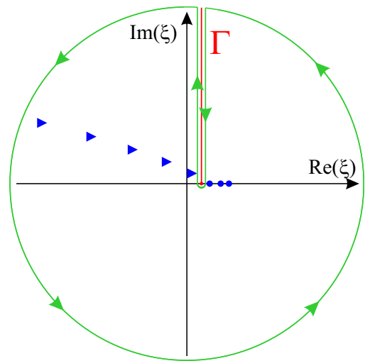
FIG. 10: “Physical” Riemann \xi -sheet. Symbols mark poles of the Green’s function G(x, x'; \xi) of the BWG. The cut \Gamma starting from the branch point at \xi = \omega^2 is shown by a red line. Green curve marks the path of integration.
