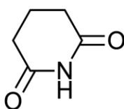
Glutarimide
