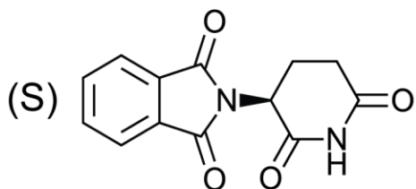
Thalidomide
