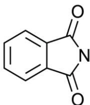
Phthalimide
