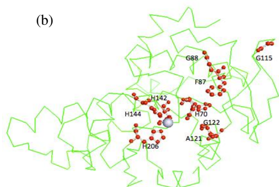
Figure 4 Catalytic site of GaFucA. A. Sequence alignment of GaFucA to 3OCR. The secondary structure elements were depicted above the alignment ( \color{red}{\sim} = \alpha -helix, \color{blue}{\sim} = \beta -strand). The active site residues are marked below the alignment by asterisks. B. Active site residues are shown in ball-and-stick (H70, F87, G88, G115, A121, G122, H142, H144, H206) representation. The grey sphere shows zinc ion.
