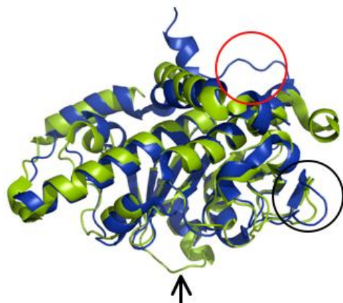
Figure 6 Superposition of the monomeric backbone of GaFucA (blue) and 3OCR (green). GaFucA had additional (red circle) and longer (black circle) loops. The arrow indicates the position of the missing loop in GaFucA.
