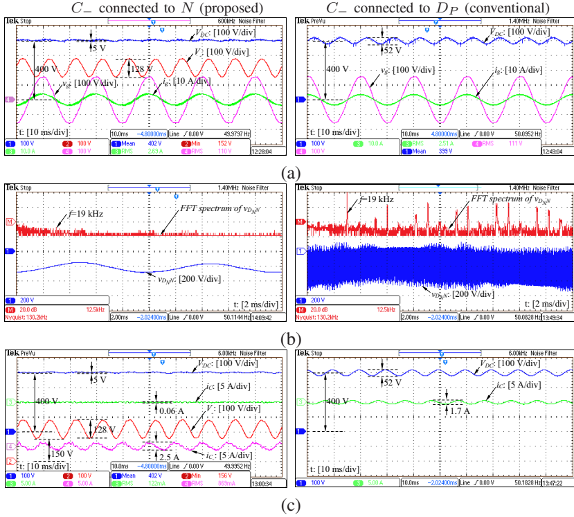
Fig. 6. Experimental results at the steady state (rectification mode): (a) Voltages V_{DC} and V_- , grid voltage v_g and current i_g ; (b) CM voltage v_{DNN} and its spectra; (c) DC voltages V_{DC} and V_- , capacitor currents i_C and i_{C-} after applying a 6 kHz low-pass filter.
