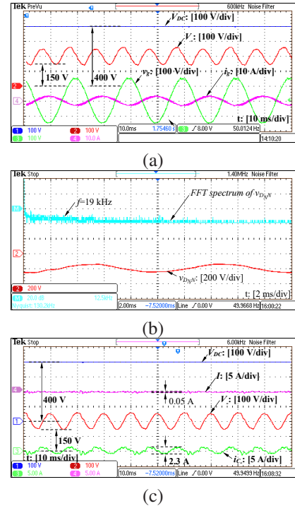
Fig. 9. Experimental results (inversion mode): (a) Voltages V_{DC} and V_- , grid voltage v_g and current i_g ; (b) CM voltage v_{D_NN} and its spectra; (c) Voltages V_{DC} and V_- , DC-bus current I and capacitor current i_{C_-} after applying a 6 kHz low-pass filter to remove the switching ripples.
