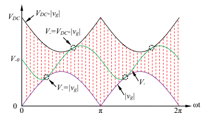
Fig. 4. Range of the voltage V_- determined by |v_g| and V_{DC} - |v_g| .
