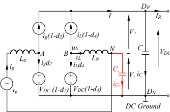
Fig. 3. Average circuit model of the proposed converter.
