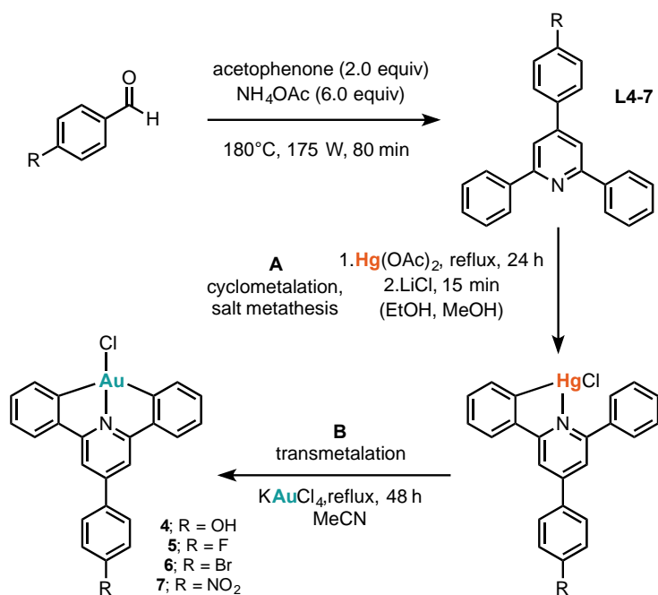
Fig. 4. Synthesis of [\text{Au(III)}(\text{C}^{\wedge}\text{N}^{\text{R}}\text{C})] ( \text{C}^{\wedge}\text{N}^{\text{R}}\text{C} = para-substituted 2,4,6-triarylpyridine) complexes.
