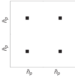
Figure 8. Deprojection matrix, \mathbf{D} : filled elements of the deprojection matrix for one pair, for one phase of data. The overall dimensions are 2\tilde{n}_p \times 2\tilde{n}_p , twice the number of pixels in a BICEP map.
