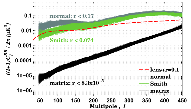
Figure 18. BB power spectra of noiseless unlensed- \Lambda CDM ( r = 0 ) simulations, estimated using various methods, demonstrating the effectiveness of the BICEP2 purification matrix. The E/B leakage using the matrix estimator is 3 orders of magnitude lower than other methods.
