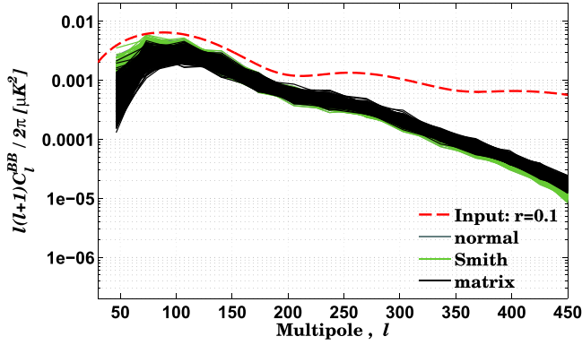
Figure 19. BB power spectra of noiseless unlensed ( r = 0.1 ) tensor only simulations, estimated using various methods. All methods suffer from loss of power due to filtering and beam effects. The removal of ambiguous modes at low l results in a further decrease in power for the matrix method. Note that the spectra in this plot have not been corrected for the beam and filter suppression factors, but in Figure 18 the correction is applied.
