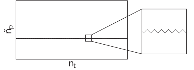
Figure 7. Pointing matrix, \Lambda : filled elements of the pointing matrix that transforms timestreams to an observed map in the BICEP pixelization. This matrix contains the mapping between the pointing of a single detector pair over one scanset and the output map pixels. There are 23,600 pixels in a BICEP map, denoted as \tilde{n}_p . There are n_t filled entries, consisting of a 1 for each timestream sample. Each leg of the zigzag pattern corresponds to a halfscan within the scanset, where the telescope is scanning back and forth at a fixed elevation.
