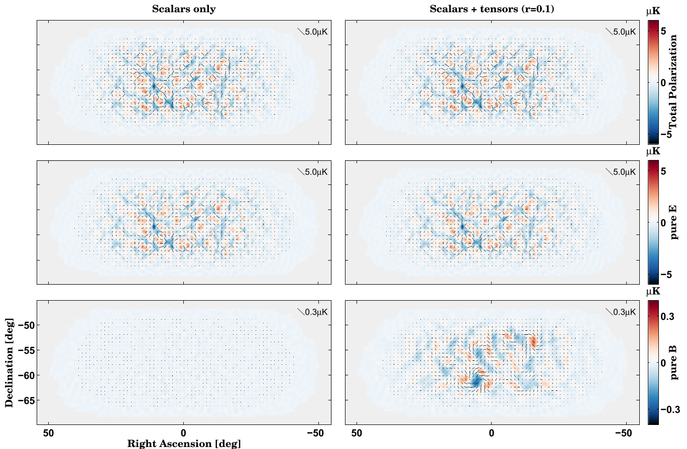
Figure 17. Polarization maps showing the effectiveness of the BICEP2 purification matrix at separating noiseless simulations into pure E and pure B . Left column: on a scalar only unlensed- \Lambda CDM BICEP2 simulation. Right Column: on the same simulation with the addition of a small tensor component. Top Row: the total polarization of the BICEP2 observed map, containing E and ambiguous modes. Center Row: pure E -mode map, constructed by projecting the total polarization map onto the E eigenmodes found in Equation (70). Bottom Row: pure B -mode map, constructed by projecting the total polarization map onto the B eigenmodes of Equation (70).
