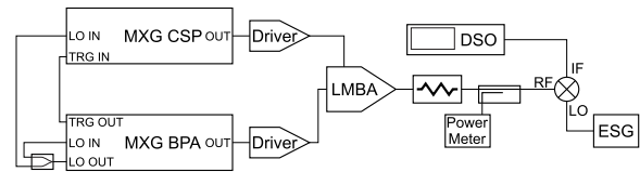
Fig. 27. Diagram of the measurement setup.
