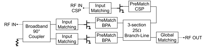
Fig. 20. Block diagram of the designed LMBA.
