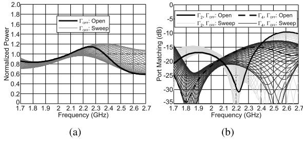
Fig. 15. Simulation results for the assessment of real coupler effect. (a) Normalized output power. (b) \Gamma_2 , \Gamma_4 , \Gamma_{\text{OFF}} = 1 (black thick line), \Gamma_{\text{OFF}} with swept phase (gray lines).
