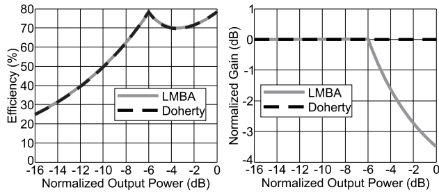
Fig. 10. (Left) Ideal drain efficiency and (right) normalized gain versus normalized output power, comparing Doherty and LMBA.
