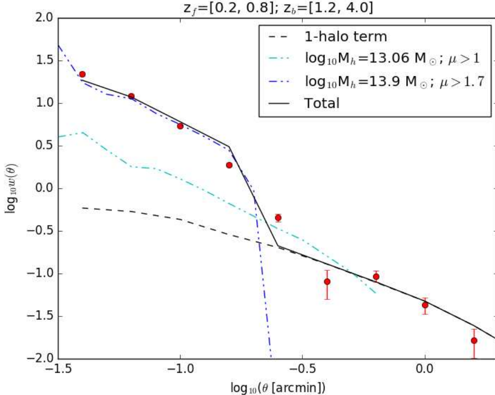
Figure 9. Toy model simulation results to confirm the strong lensing regime interpretation. The measured angular cross-correlation using the default foreground lensing sample ( red circles ) is fitted with the 1-halo term under the weak lensing approximation ( black dashed line ) plus a contribution of the strong lensing effect, \mu > 1.7 , produced by massive halos, \log_{10}(M_{\text{halo}}/M_{\odot}) = 13.9 , estimated using the simulations described in the text ( blue dot-dot-dashed line ). The simulations results, considering all amplifications, for the derived M_{\text{min}} is shown as well ( cyan dot-dot-dashed line )
