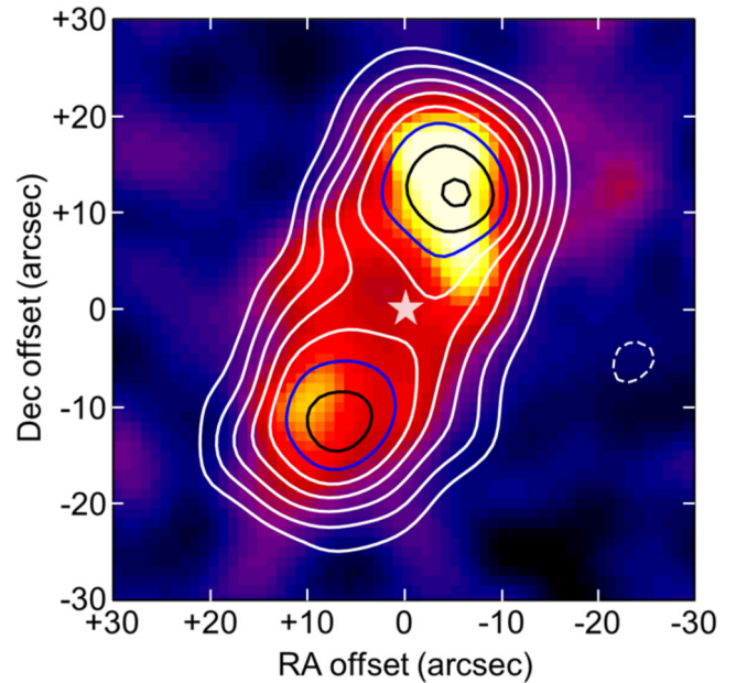
Figure 25. The 450 \mu m S/N image from observations of Fomalhaut (HD 216956) with contours from the 850 \mu m image overlaid. The colours are scaled from -3\sigma to the maximum S/N in the image. The contours start at -5\sigma (dashed white) and then solid colours from 5\sigma to the maximum in 5\sigma steps. The star symbol represents the position of the star with respect to the disc.
