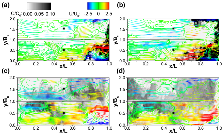
Fig. 13 Normalised tracer concentration contours ( C/C_0 ) and super-imposed flow streamlines ( U/U_b ) on a horizontal plane ( z/H = 0.65 ) extracted at the middle of the first ( y/B_c < 1 ) and second ( y/B_c > 1 ) chambers. a t = 27 s ( \theta = 0.021 ), b t = 36 s ( \theta = 0.028 ), c t = 102 s ( \theta = 0.08 ), and d t = 124.5 s ( \theta = 0.099 ). Black squares represent the sampling points location
