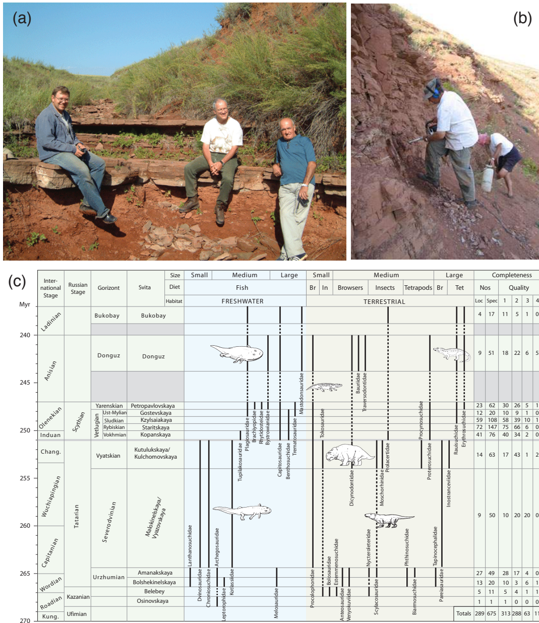
Figure 5. The Permo-Triassic boundary in Russia. (a) The Kulchomovskaya Svita (latest Permian) below the ledge, and the Kopanskaya Svita (basalmost Triassic) above, in the Korolki Ravine, near Sol-Iletsk, on the south-western margin of the Urals, Asiatic Russia. Mikhail Surkov, M.J.B. and Valentin Tverdokhlebov inspect the sandstone lying right at the boundary. (b) Graeme Taylor drills rock plugs for magnetostratigraphic analysis in the Boyevaya Gora PTB section, South Urals, assisted by M.J.B. (c) Overview of the fates of tetrapods from the Middle Permian to Middle Triassic, showing that only procolophonids and dicynodonts survived the Permo-Triassic mass extinction.
