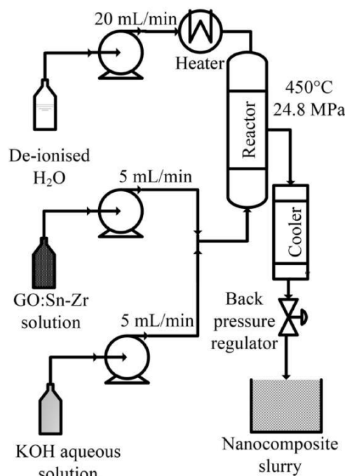
Fig. 2. Schematic of a CHFS reactor set-up used for the synthesis of Zr-Sn/graphene nanocomposite catalyst.
