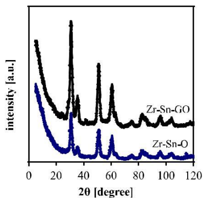
Fig. 4. X-ray powder diffraction (XRD) patterns of tin doped zirconium oxide (Zr-Sn-O) (b) tin doped zirconia/graphene nanocomposite (Zr-Sn/GO).
