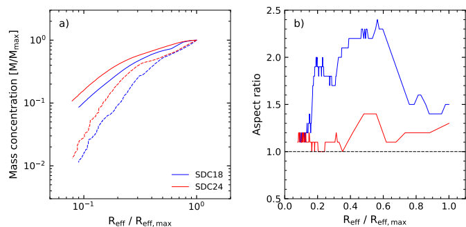
Fig. 12. a) the concentration of mass as a function of radius within the two IRDCs. The solid and dashed lines show the upper and lower limits on the mass, respectively, as in panel d) of Fig. 11. b) the aspect ratio (as defined by Peretto & Fuller 2009) of each structure as a function of the normalised effective radius.
