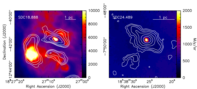
Fig. 14. Herschel 70 \mu\text{m} images of SDC18 (left) and SDC24 (right) from the Hi-GAL survey. Note the bright 70 micron sources at the locations of the column density peaks. The contours show the 2.0 mm SNR as in Fig. 5.
