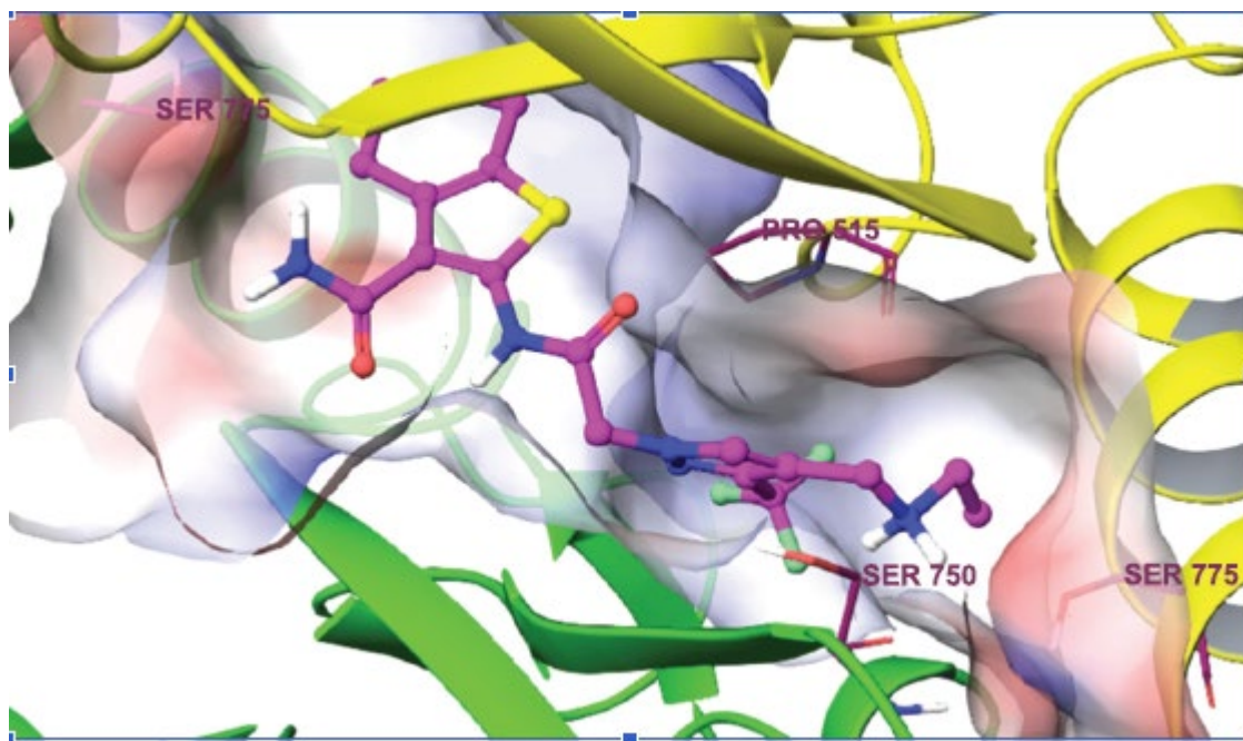
Fig. (24). X-ray structure of 73 ( R_1 = \text{Et} , R_2 = \text{H} ) in complex with the S1S2 LBD of hGluA2i (PDB code 3O6H, 2.1 Å resolution).
