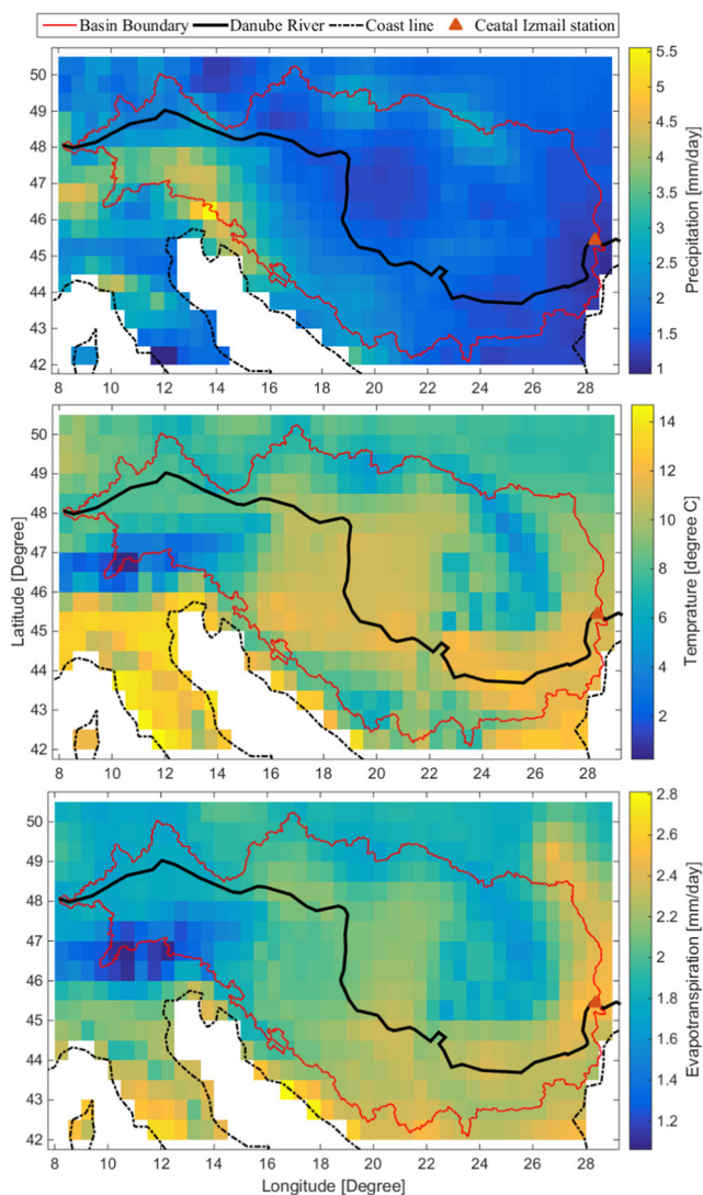
Fig. 4 Average precipitation (mm/day), average temperature ( ^{\circ}\text{C} ) and average evapotranspiration (mm/day) within the Danube River Basin during the study period (2000–2010). The red line defines the basin's boundary, the black line represents the Danube River. The red triangle represents the Ceatal Izmail station position. X and Y axes represent the longitude and latitude in degree ( ^{\circ} ), respectively
