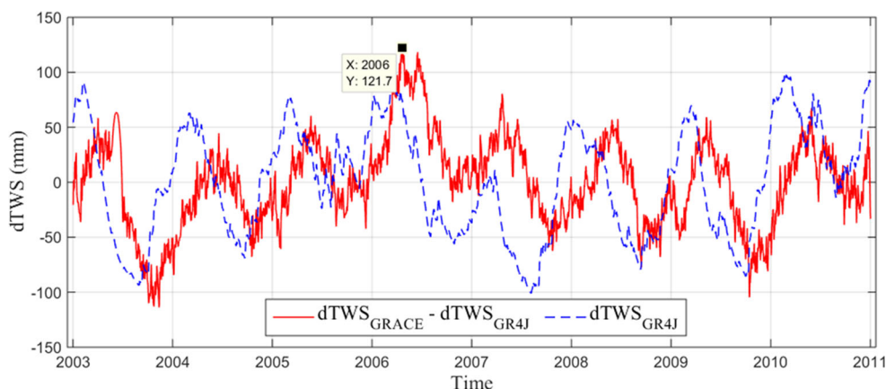
Fig. 6 Daily TWS (dTWS) anomalies simulated by GR4J within the Danube River Basin during January 2003 to December 2010. We used 161.32, 13.43, 914.18 and 12.08 for X1 to X4, respectively, that are estimated by calibrating GR4J against (only) runoff observations.
