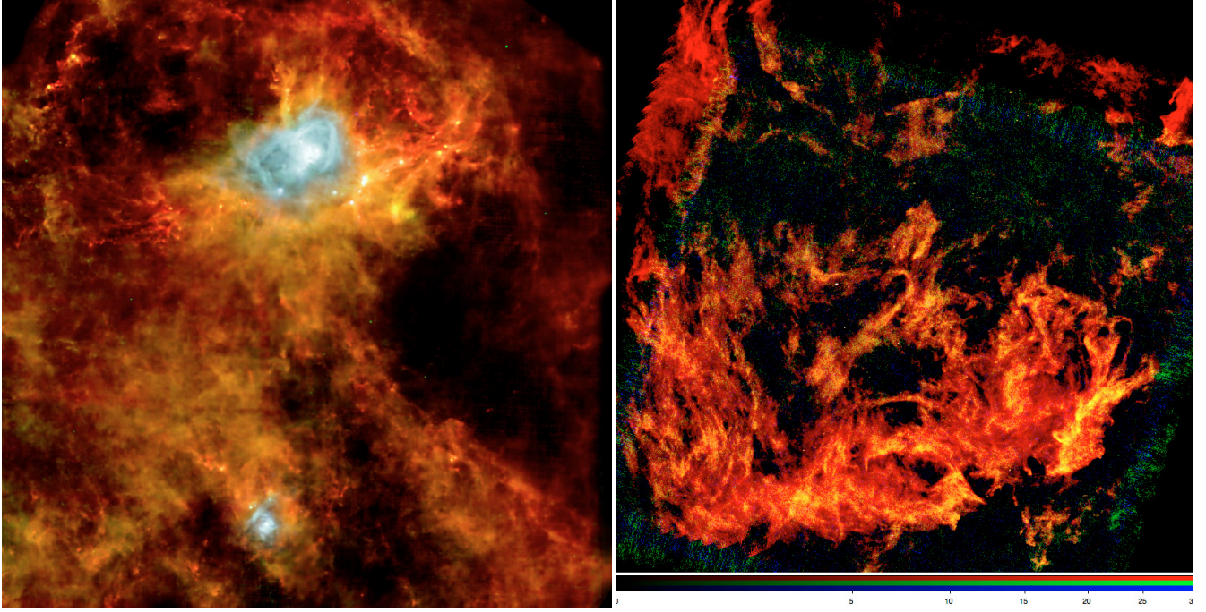
Fig. 3. Composite 3-color images of the \sim 11 deg 2 Aquila field ( left ) and the \sim 8 deg 2 Polaris field ( right ) produced from our PACS/SPIRE parallel-mode images at 70, 160, and 500 \mu\text{m} . The color coding of the Aquila image is such that Red = SPIRE 500 \mu\text{m} , Green = PACS 160 \mu\text{m} , Blue = PACS 70 \mu\text{m} . For the Polaris image, Red = combination of the three SPIRE bands, Green = PACS 160 \mu\text{m} , Blue = PACS 70 \mu\text{m} . The Aquila composite image was also the first release of “OSHI”, ESA’s Online Showcase of Herschel Images (cf. http://oshi.esa.int and http://www.esa.int/SPECIALS/Herschel/SEMT0T9K73G_0.html ).
