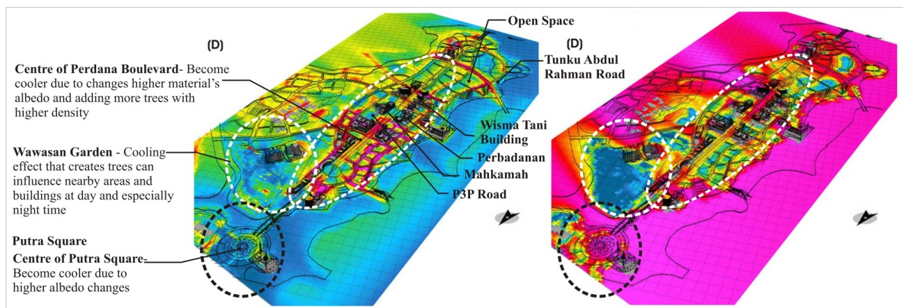
Figure 5.45 Predicted air temperatures in condition (D) where larger cooling effects can be found throughout the Persiaran Perdana area due to trees and ground material modifications (right) at 15:00; (left) at 03:00.
