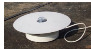
Figure 4.30 Pyranometer with base and screen model CM – CM 5
