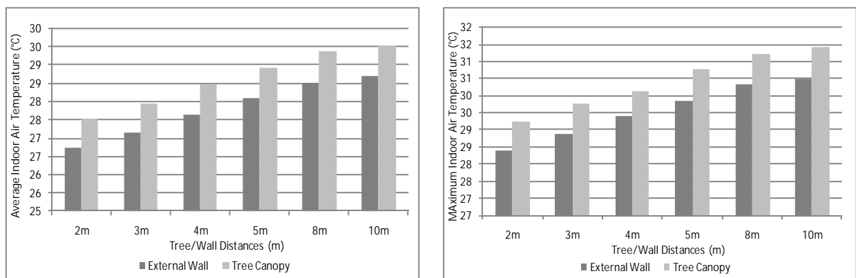
Figure 7.4 Comparison of external wall and tree canopy on average (left) and maximum (right) indoor air temperature at distance variation
