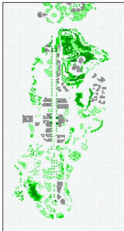
Figure 4.41 The 1D main model domain of Persiaran Perdana in a grid cell
