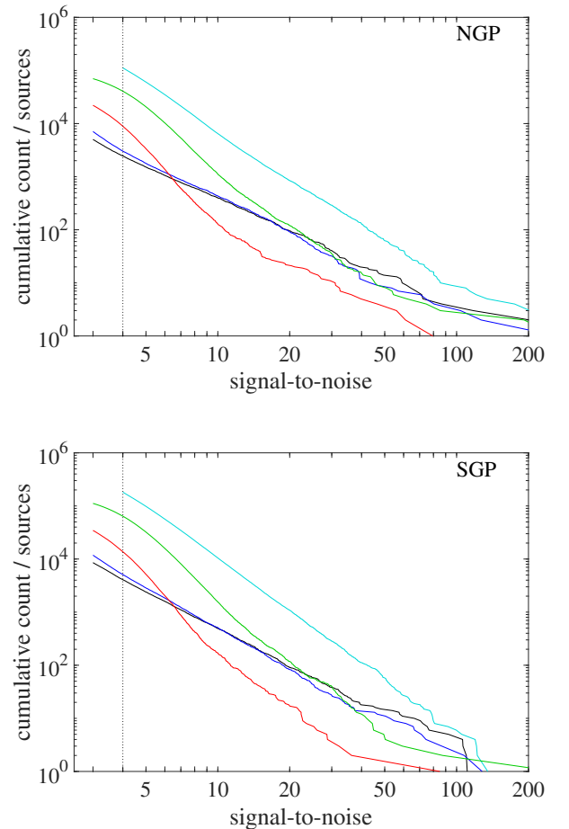
Figure 7. The cumulative number of sources as a function of signal-to-noise at 100 \mu\text{m} (black), 160 \mu\text{m} (blue), 250 \mu\text{m} (cyan), 350 \mu\text{m} (green) and 500 \mu\text{m} (red). The NGP area is shown in the top panel, and the SGP in bottom panel. The vertical dotted line shows the 4\text{-}\sigma limit for the 250 \mu\text{m} selection. The other bands are truncated at 3\text{-}\sigma .
