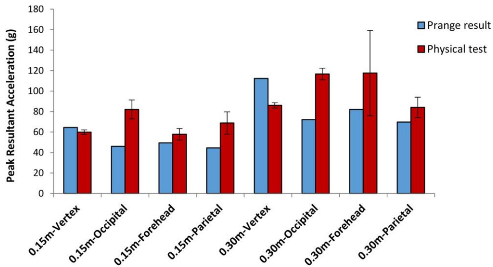
Fig. 5. Peak acceleration and drop height for infant PMHS and physical model impact tests.
