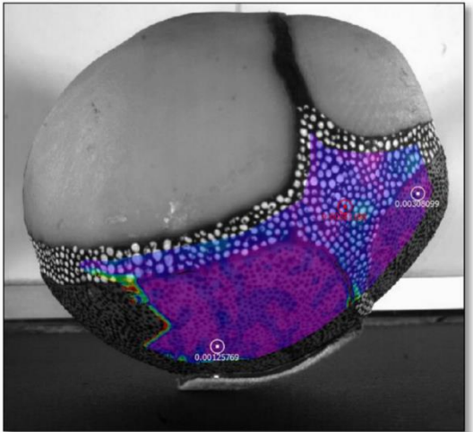
(c) Parietal impact test
