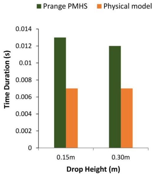
Fig. 6. Comparison of impact time duration between PMHS test and physical model.
