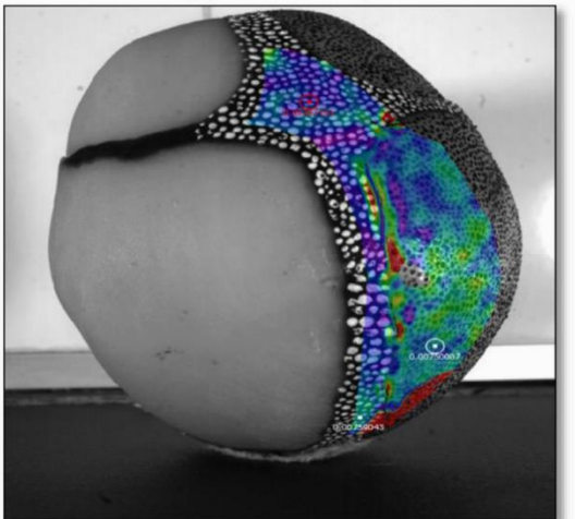
(e) Occipital impact test
