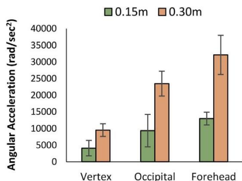
Fig. 9. Physical model maximum angular acceleration from different impact locations at two drop heights.
