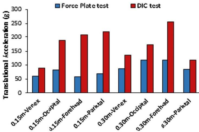
Fig. 8. Physical model comparison of translational acceleration from the force plate and DIC system.
