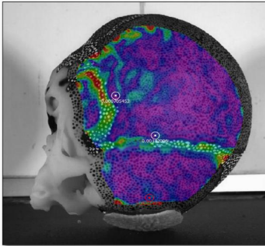
(a) Forehead impact test
