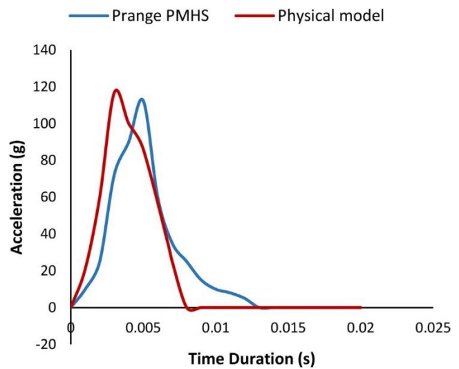
Fig. 7. Acceleration–time contact curve for the forehead area from a 0.30 m height drop.
