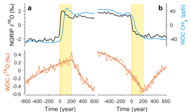
Fig. 2. Time relationships between Greenland and Antarctic ice-core data during Marine Isotope Stage 3. a) Stacked data from DO 3–18 of NGRIP \delta^{18}\text{O} (black), WDC methane (blue) and WDC \delta^{18}\text{O} (orange curve with fit), aligned at the mid point of the NGRIP interstadial transitions; on average Antarctica begins cooling 218 \pm 92 years after each Greenland interstadial warming transition. b) As for a) but for NGRIP stadal transitions; on average Antarctica begins warming 208 \pm 96 years after each Greenland stadal cooling transition. The errors denote 95% confidence levels accounting for dating and procedural uncertainties. WDC data is from WAIS Divide Project Members (2015), NGRIP data from North Greenland Ice Core Project members (2004). Figure adapted from WAIS Divide Project Members (2015).
