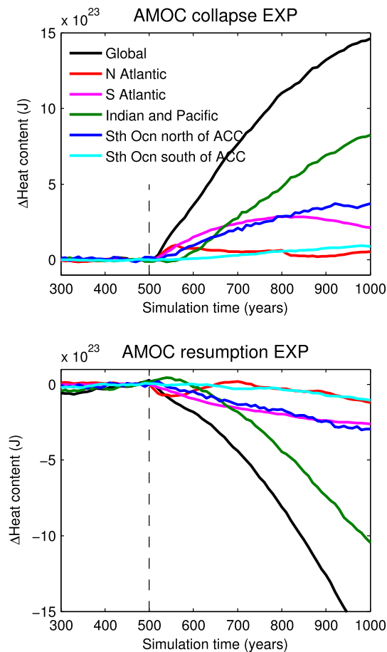
Fig. 6. Modelled changes in heat content of the global ocean and of specific ocean regions during the AMOC collapse (top) and AMOC resumption (bottom) experiments. Dashed vertical lines mark the start of the AMOC perturbations. We take 40°S as the northern boundary of the Southern Ocean.
