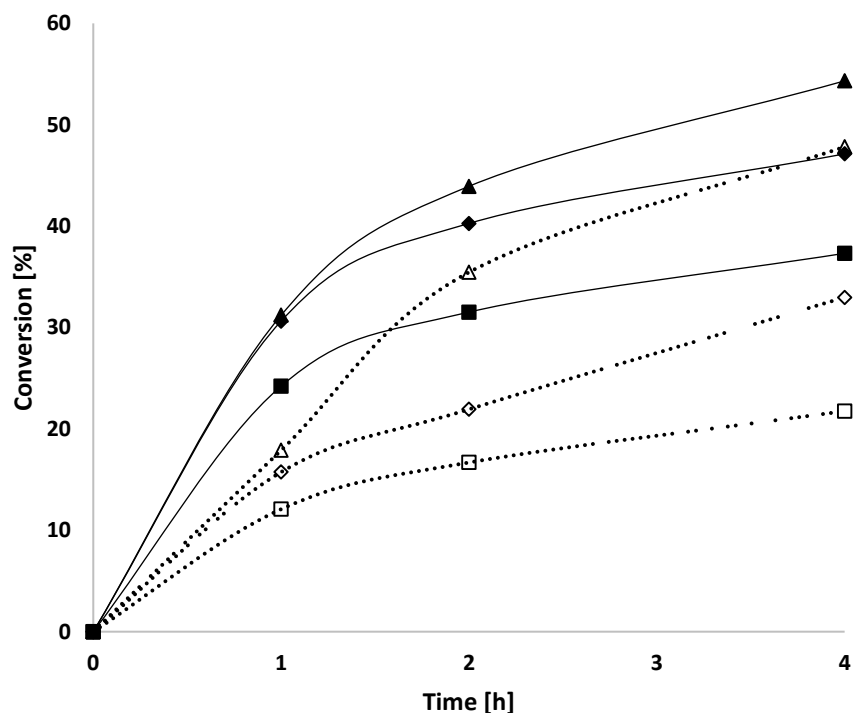
ESI Figure 1 Oxidation of cinnamyl alcohol under different oxygen pressure carried out in the presence and absence of the catalyst as a function of reaction time. Reaction conditions: 1%AuPd/TiO 2 (Imp), 10 mg; oxygen pressure, 1-3 bar; temperature, 120 °C; 0.5 M cinnamyl alcohol in toluene. Full figures- reactions carried out in the absence of a catalyst: 1 bar (■); 2 bar (◆), 3 bar (▲); empty figure- reactions carried out in the presence of a catalyst: 1 bar (□); 2 bar (◇); 3 bar (△)
