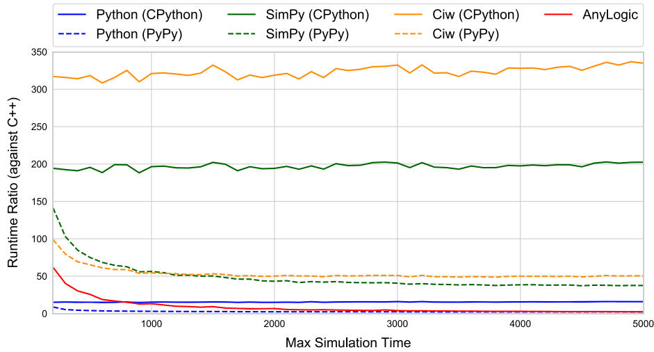
Figure 9. Comparison between the runtimes of the C++ model, bespoke Python Ciw model, the SimPy model, the Ciw model and the AnyLogic model.
