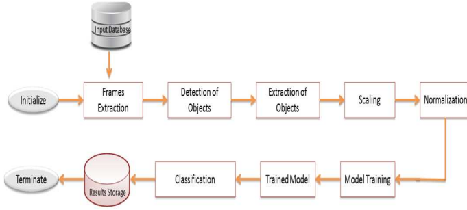
Fig. 3: Workflow of the Proposed Network
