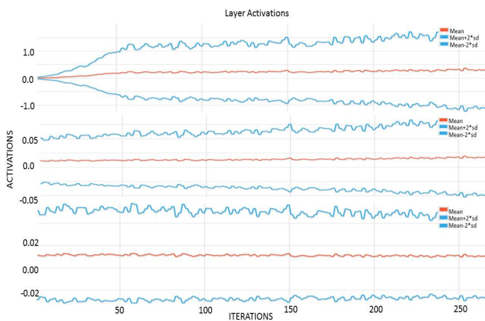
Fig. 8: Layer Activations
