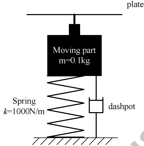
Fig. 2 Dynamic model of the electromagnetic shaker
