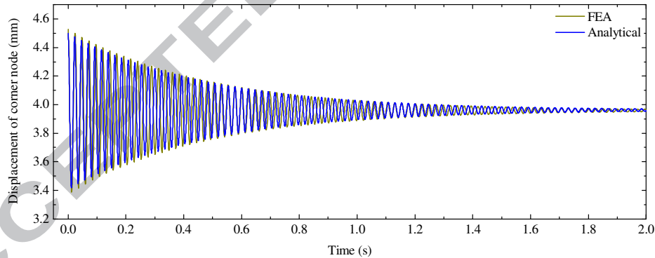
Fig. 9 Predicted free vibration of the 100mm \times 100mm, [0_3/90_3]_T plate with the proportional damping coefficient \alpha = 100
