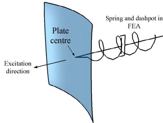
Fig. 4 Schematic of the finite element model of the plate and shaker system
