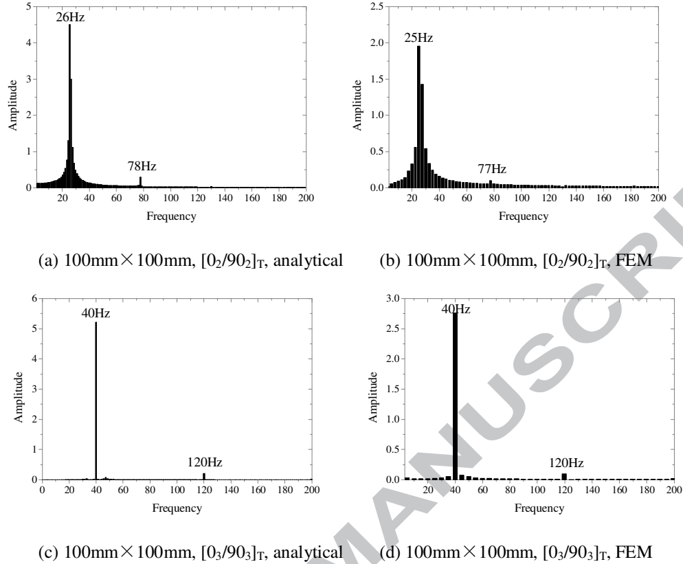
Fig. 17 FFT of the corner displacements in Fig. 16
