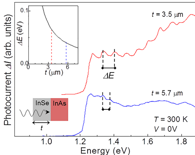
FIG. 2. Photocurrent spectra for two n -InAs/ p -InSe heterojunctions at V = 0 \text{ V} and T = 300 \text{ K} . The insets show the calculated dependence of the periodicity \Delta E of the interference pattern seen in the spectra on the thickness t of the p -InSe layer. As sketched in the inset, light propagates in the direction perpendicular to the layers of the heterojunction.
