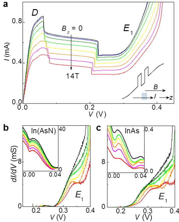
Figure 4. Resonant Zener tunnelling in magnetic field parallel to the direction of current. (a) Current-voltage I(V) curves at magnetic fields B_z = 0, 2, 4, 6, 8, 10, 12, 14 T, applied parallel to the direction z of the current for an In(AsN) RTD with mesa diameter d = 100 \mu\text{m} ( T = 2 K). (b,c) Differential conductance dI(V)/dV curves versus B_z in the bias region of electron tunnelling into the first subband, E_1 , of the In(AsN) (b) and InAs (c) QW for B_z = 0, 4, 6, 8, 10 , and 14 T. The insets show the dI(V)/dV curves at small applied biases ( T = 2 K).
