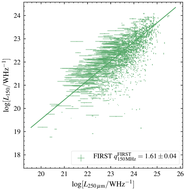
(b) The FIRC as measured with FIRST at 1.4GHz
