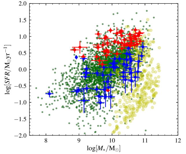
Figure 15. Stellar mass versus star formation rate for our sample. Our full sample is plotted in green. The 100 galaxies selected from both the WISE-red sub-sample (red) and the WISE-blue sub-sample (blue) are shown as the larger points with errorbars. For comparison, AGN classified by BPT are plotted in yellow.
