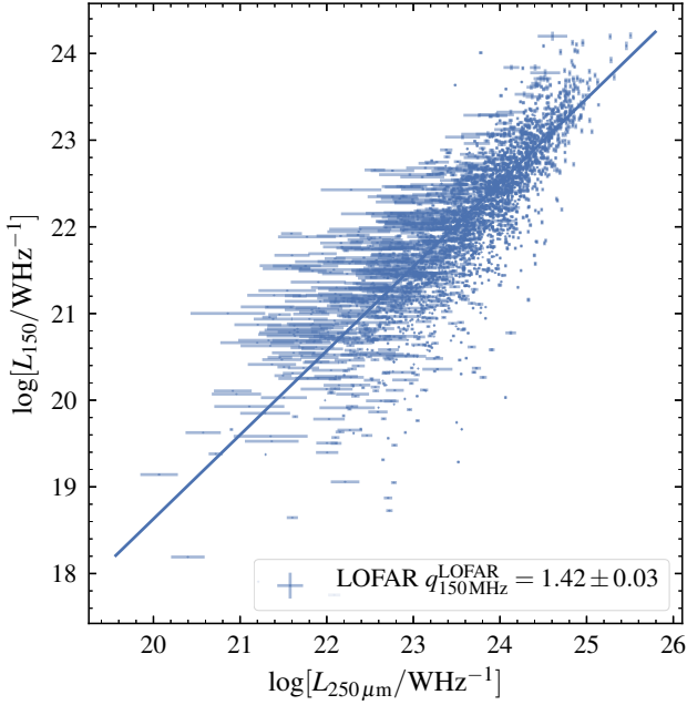
(a) The FIRC as measured with LOFAR at 150MHz
