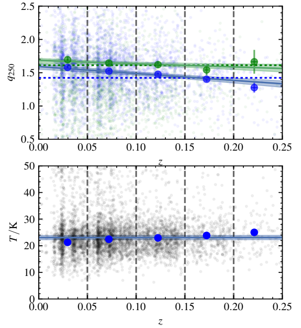
Figure 8. Top: Evolution of q_{250} over redshift measured with LOFAR at 150MHz (blue) and FIRST transformed to 150MHz (green). The dashed horizontal line in the upper plot is the mean-stacked q_{250} for all star-forming galaxies taken from Figure 6 for FIRST and LOFAR at 150MHz. The coloured lines indicate the straight line fit to all galaxies in our sample binned in redshift for LOFAR and FIRST. Bottom: The temperature in each bin, calculated by constructing an infrared SED from the average K -corrected flux of each source in every band and fitting Equation 2 to the result. The temperature and uncertainties are overlaid with a straight line fit to the data. The vertical dashed lines represent bin edges.
