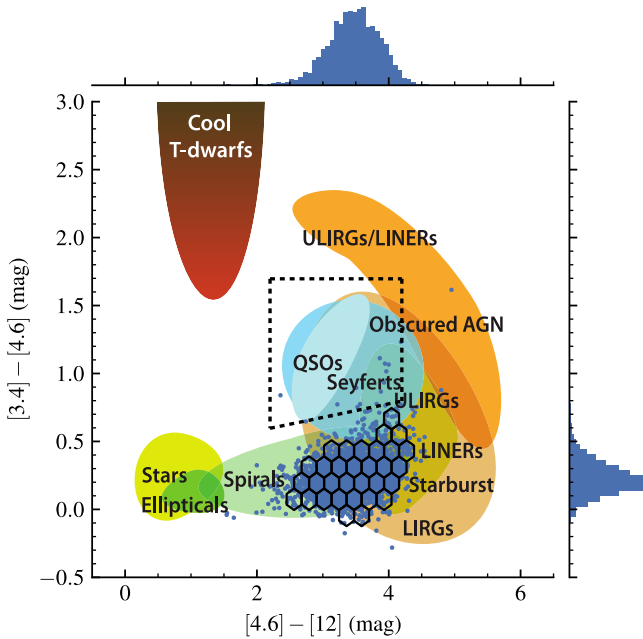
Figure 2. The mid-infrared sub-sample ( 5\sigma WISE detections, shown as blue points) overlaid on the Jarrett et al. (2011) MIRDD which uses the magnitudes at three WISE wavelengths W1 at 3.4\ \mu\text{m} , W2 at 4.6\ \mu\text{m} , and W3 at 12\ \mu\text{m} . The coloured regions are as published in Wright et al. (2010), and intended to show the approximate locations of galaxies of a range of different types. The hexagonal bins over the region centred on [4.6] - [12] \approx 3.5 , and [3.4] - [4.6] \approx 0.25 are used to trace q_{250} in later sections of this paper, and are shown here to provide context. The QSO box defined by (Jarrett et al. 2011) is depicted as a dashed box. Number counts over both colours are shown as blue histograms.
