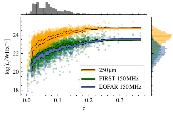
Figure 7. Distributions of Herschel SPIRE 250 \mu\text{m} (yellow), FIRST (green), and LOFAR (blue) luminosity densities over redshift for our main star-forming sample. A rolling mean (inclusive of all non-detections) with a window size of 200 points is plotted to guide the eye.
