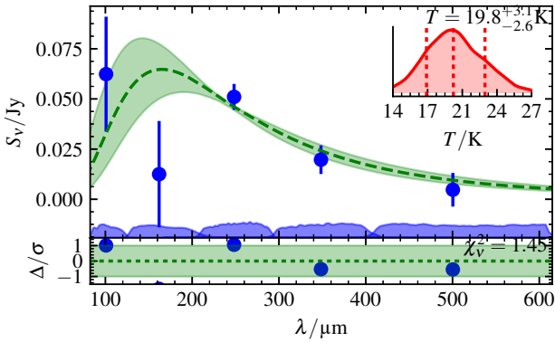
Figure 4. A sample isothermal fit to an SDSS star-forming galaxy at \alpha_{J2000} = 12^h49^m46.1^s , \delta_{J2000} = 31^\circ35'30'' . The probability distribution for temperature is shown in the top right with the 1-sigma equal-tailed credible interval as dashed lines around the median temperature of 19.8K with a reduced \chi^2 of 1.45. The Herschel flux measurements and their uncertainties are shown as blue errorbars. The fit observed-frame isothermal greybody with its own 1\sigma credible interval is shown as the green curve. The differences between the estimated flux and the measurement are shown along the bottom axis. The filter transmission profiles are also shown in blue along the bottom for each wavelength.
