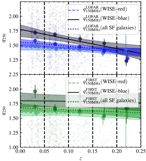
Figure B3. Evolution of q_{250} over redshift for the WISE-red (light points, dashed lines), WISE-blue (darker points, solid lines), and all star-forming galaxies (dotted line) measured with LOFAR at 150MHz (blue) and FIRST transformed to 150MHz (green). The coloured lines indicate the straight line fit to all galaxies in our sample binned in redshift for LOFAR and FIRST.
