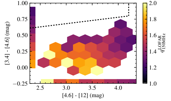
(a) LOFAR at 150 MHz
