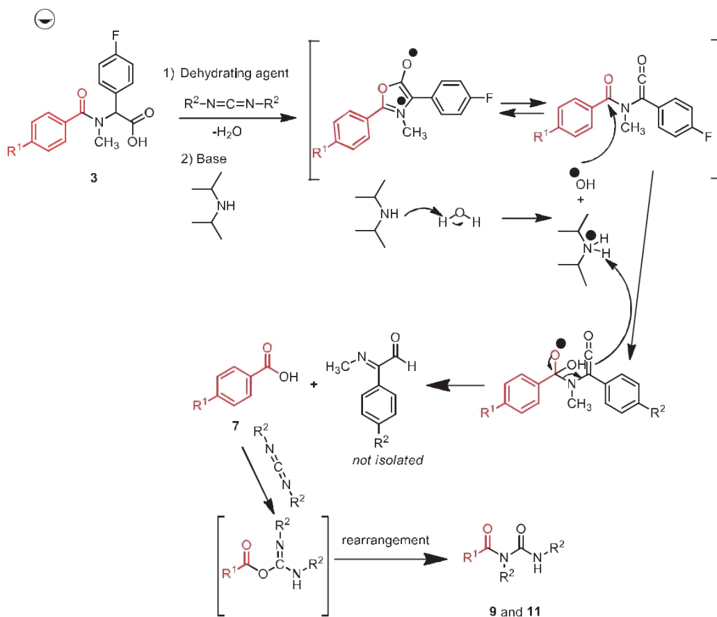
Scheme 7. A plausible reaction mechanism leading to N-acylureas 9 and 11.
