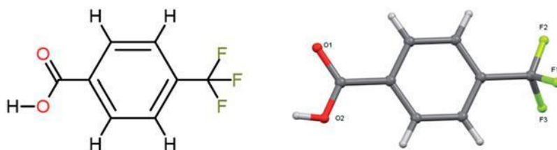
Figure 4. X-Ray ORTEP view of 7f.
