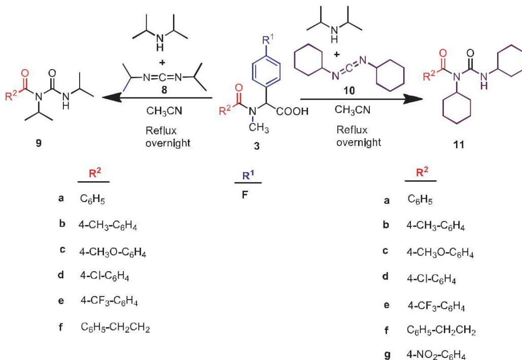
Scheme 6. Reactions of munchnone€ precursors 3 with diisopropyl carbodiimide (DIPC) 8 and dicyclohexyl carbodiimide (DCC) 10 in the presence of diisopropyl amine (DIPA) to afford 9a-f and 11a-g . Reagents and solvent: 3 (0.47 mmol), 8 (3.0 mL), 10 (1.91 mmol), DIPA (0.2 mL), CH 3 CN (10.0 mL).
