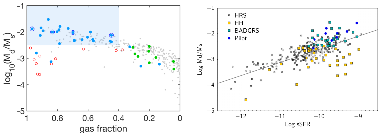
Figure 1. Left: Specific dust mass ( M_d/M_* ) versus gas fraction for local galaxy samples. Galaxies with \text{FUV} - \text{K} < 3.5 and which are detected in H-ATLAS are denoted by blue circles. The parent samples are the dust-selected local volume sources from Clark et al. (2015) and the H I-selected sample from De Vis et al. (2017a). Dust- and H I-selected sources from the parent samples which do not have both the blue colour and H-ATLAS detections are shown as filled green and red open circles, respectively. The shaded box indicates our definition of BADGRS as described in the text. Our CO BADGRS sample is highlighted by dark blue circles surrounding the points. K-band-selected sources (grey) are from HRS (Boselli et al. 2010). Dust masses are all scaled to \kappa_{250} = 0.56 \text{ m}^2 \text{ kg}^{-1} and are determined in an equivalent way, using either MAGPHYS or two temperature MBB fitting. For more information on dust mass determination, see Section 4. Right: Dust mass versus SFR (normalized by stellar mass). BADGRS have more dust per unit SFR than typical galaxies and the wide spread of dust per SFR is apparent at high sSFR due to the inclusion of the H I-selected, dust-poor sources from HIGH (De Vis et al. 2017a). BADGRS from both HIGH and HAPLESS are shown in cyan while the individual regions of the pilot sample presented here are blue circles. Gold squares are the HIGH and HAPLESS sources which do not meet the BADGRS criteria of being blue and dusty.
