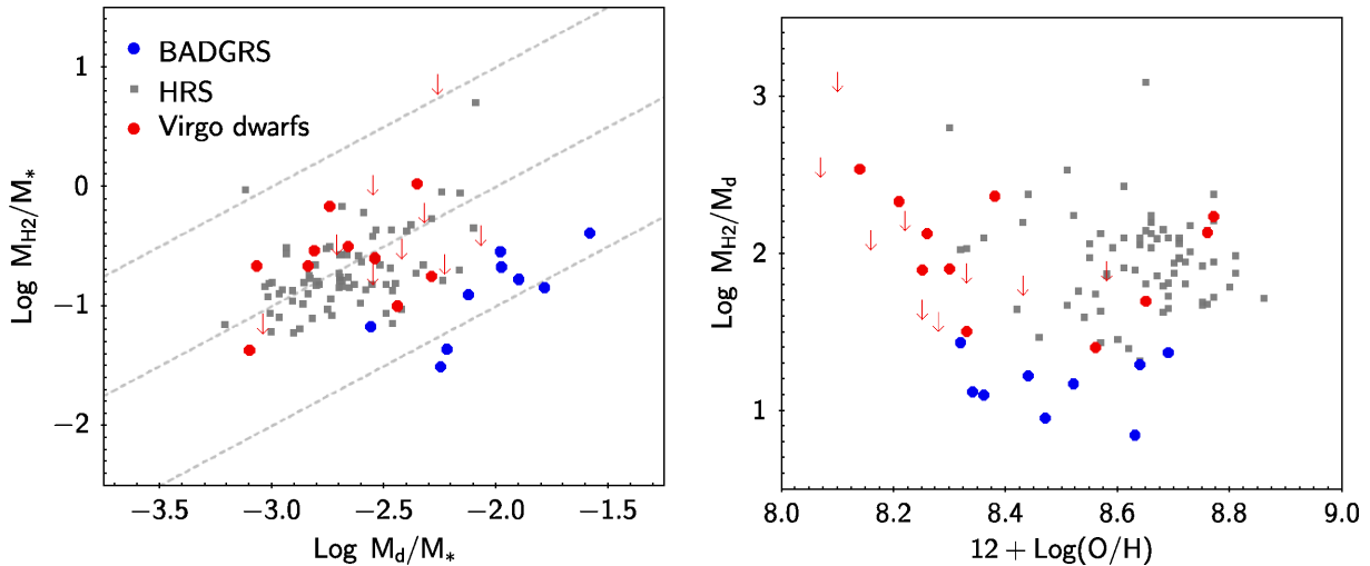
Figure 5. (a) The correlation between dust and molecular gas mass having normalized by the common scaling factor of stellar mass. The dashed lines indicate constant M_{\text{H}_2}/M_{\text{d}} ratios of 10, 100, and 1000 (bottom to top). BADGRS are the most dust-rich (relative to M_* ) galaxies and lie below the extrapolated trend for M_{\text{H}_2}/M_{\text{d}} from the other samples. (b) Molecular gas to dust ratio as a function of metallicity. There is no correlation, but BADGRS lie clearly below the average M_{\text{H}_2}/M_{\text{d}} ratios for the other samples. Metallicities are all in the O3N2 calibration of Pettini & Pagel (2004). Dust masses for the HRS are from MAGPHYS (De Vis et al. 2017a), while dust masses for Virgo dwarfs are scaled from the \beta = 2 version in Grossi et al. (2016) to be comparable to MAGPHYS as follows. The HRS MAGPHYS dust masses were compared to those determined by Grossi et al. (2016) using their single MBB \beta = 2 method. A tight correlation with linear slope, and an offset of \text{Log}(M_{\text{d,MP}}/M_{\text{d,G16}}) = 0.23 dex was found (once all were scaled to the same \kappa_{\text{d}} ). This difference is due to MAGPHYS fitting a more realistic temperature distribution which captures better the colder dust component. We scale the Virgo dwarf dust masses up by this amount to be consistent with HRS and BADGRS. All dust masses are scaled to a common \kappa_{250} = 0.56 \text{ m}^2 \text{ kg}^{-1} .
