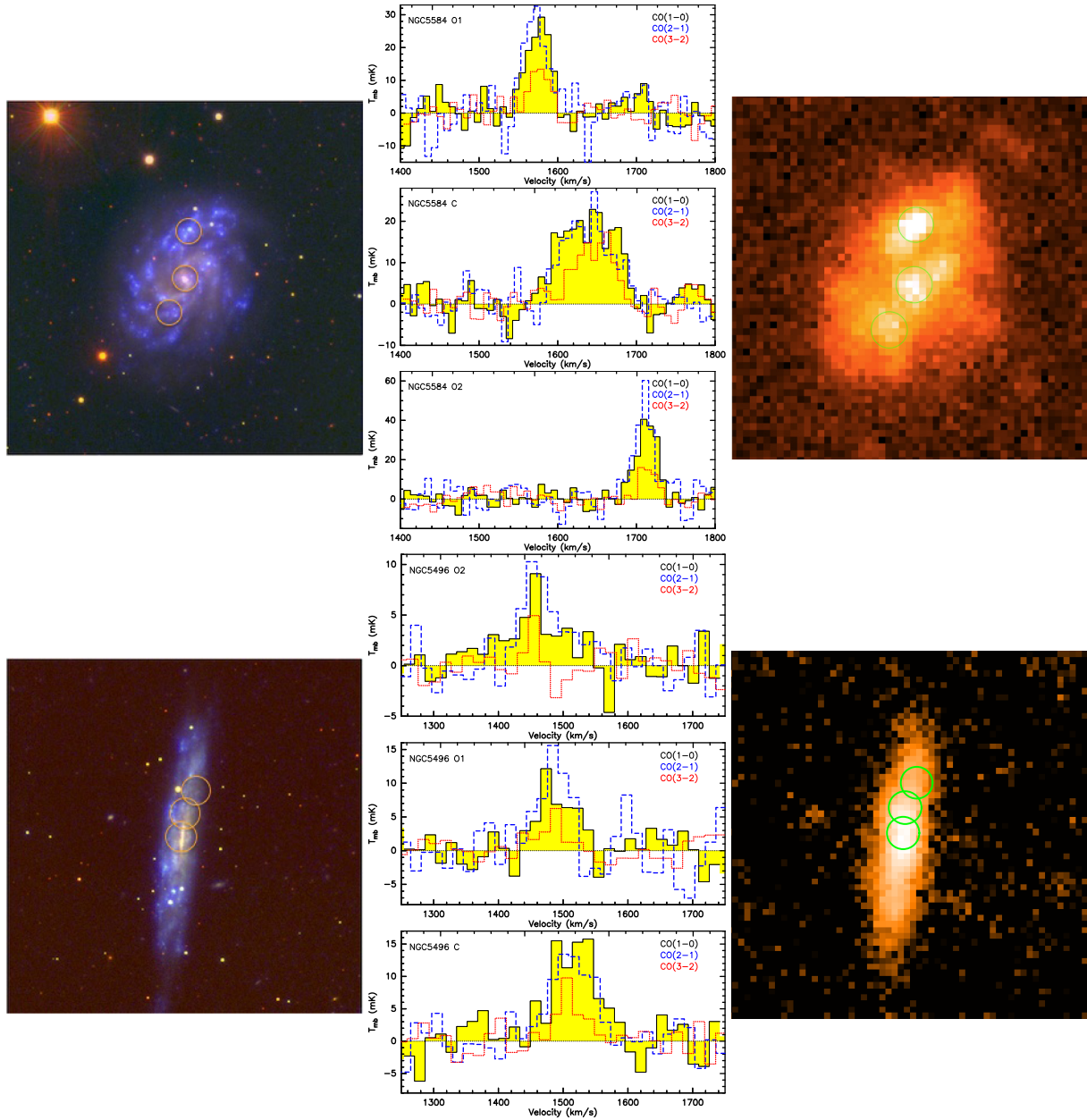
Figure 2. Left: NUV/ r/Z composite image of NGC 5584 (top) and NGC 5496 (bottom) with the CO pointings shown in yellow, representing the FWHM of the ^{12}\text{CO}(1-0) beam (22 arcsec). Centre: Spectra on the T_{\text{mb}} scale for each pointing, all three transitions are included in each panel. Right: The 250 \mu\text{m} image (un-smoothed) with the CO pointings shown. Left: NUV/ r/Z composite image of UGC9215 (top) and UGC9299 (bottom) with the CO pointings shown in yellow, representing the FWHM of the ^{12}\text{CO}(1-0) beam (22 arcsec). Centre: Spectra on the T_{\text{mb}} scale for each pointing, all three transitions are included in each panel. Right: The 250- \mu\text{m} image (un-smoothed) with the CO pointings shown.
