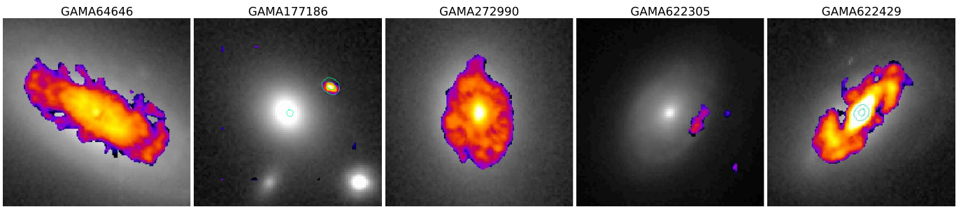
Figure 7. Composite images for the central 17'' by 17'' regions of our five target galaxies, centred on the optical position of the galaxies. Greyscale plots show KiDS r-band images with logarithmic scaling. Coloured overlays show the ALMA moment zero line emission as in Figures 3 and 4 above, with colour representing intensity in this figure. Green contours indicate the ALMA continuum emission near the centre of GAMA177186, its offset source at 4.4'' north west of the target, and near the centre of GAMA622429.
