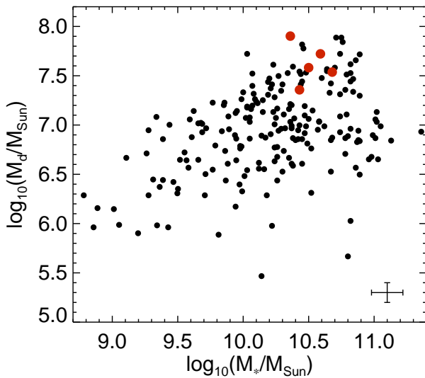
Figure 2. Log of dust mass, \text{Log}(M_d) , plotted against log of their stellar mass, \text{Log}(M_*) , for the parent sample of H-ATLAS detected ETGs (from Agius et al. 2013), in solar units. Our five target galaxies with ALMA observations are highlighted as larger filled red symbols.
