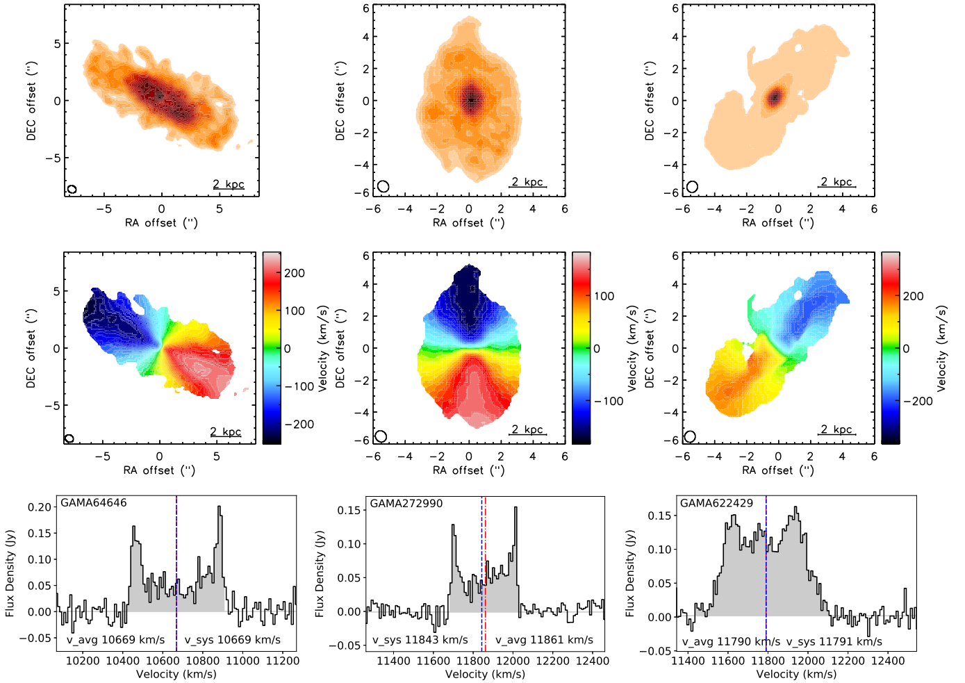
Figure 3. Moment maps and spectra for GAMA64646, GAMA272990 and GAMA622429 from left to right. Upper row: ^{12}\text{CO}(2-1) line emission images from ALMA Band 6 central observations, with scale shown. Regions with fluxes above 1.5 \times the rms noise are shown. Middle row: ^{12}\text{CO}(2-1) first order moment maps showing velocities of gas in detected target galaxies, again with scale shown. Lower row: Spectra of the ^{12}\text{CO}(2-1) emission line in each galaxy. The red dot-dashed line is the mean velocity for the channel range selected and the blue dashed line is the systemic velocity of the target galaxy in each case.
