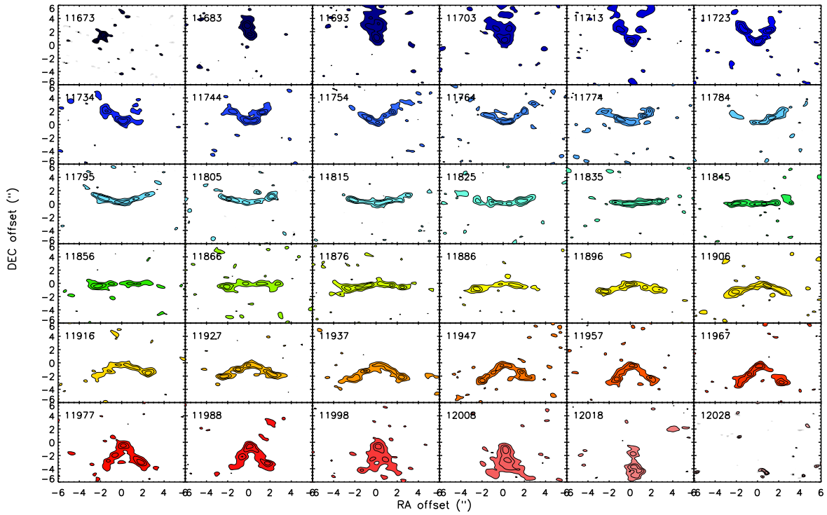
Figure A2. Channel maps for GAMA272990 showing the extended CO emission from this galaxy, across its detected velocity channels. The central velocity is shown top left in each channel map, in \text{km s}^{-1} .
