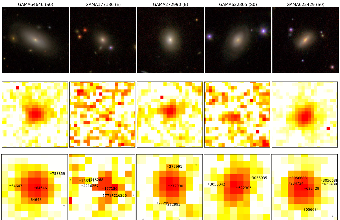
Figure 1. All images are approximately 1 arcminute by 1 arcminute, with north at the top and east on the left. Upper row: KiDS BGR composite images of these five galaxies (processed by Lee Kelvin at ARI/LJMU to a common zero point and gain). Middle row: H-ATLAS PACS 100\mu\text{m} images ( 3'' per pixel). Lower row: H-ATLAS SPIRE 250\mu\text{m} images of these five galaxies ( 6'' per pixel), illustrating their strong submm detections in H-ATLAS, centred on the optical galaxy. GAMA IDs are indicated in these fields.
