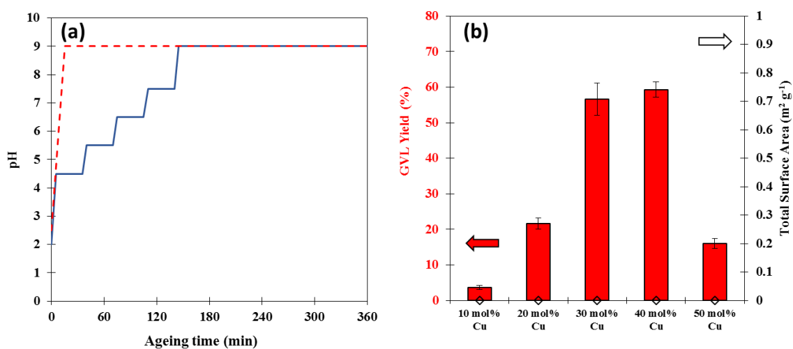
Fig. 1. A series of \text{Cu-ZrO}_2 catalyst with varied \text{Cu/Zr} loadings were prepared via a pH gradient methodology (a); the dotted and solid lines correspond to the pH ramp in the standard and pH gradient methods, respectively. The activity of the catalysts for the hydrogenation of LA to GVL and their total surface area as determined by BET is displayed in (b). Reaction conditions: 200^\circ\text{C} ; \text{H}_2 27 bar; 2 h; substrate 5 wt% LA/ \text{H}_2\text{O} (10 g); catalyst (0.05 g).
