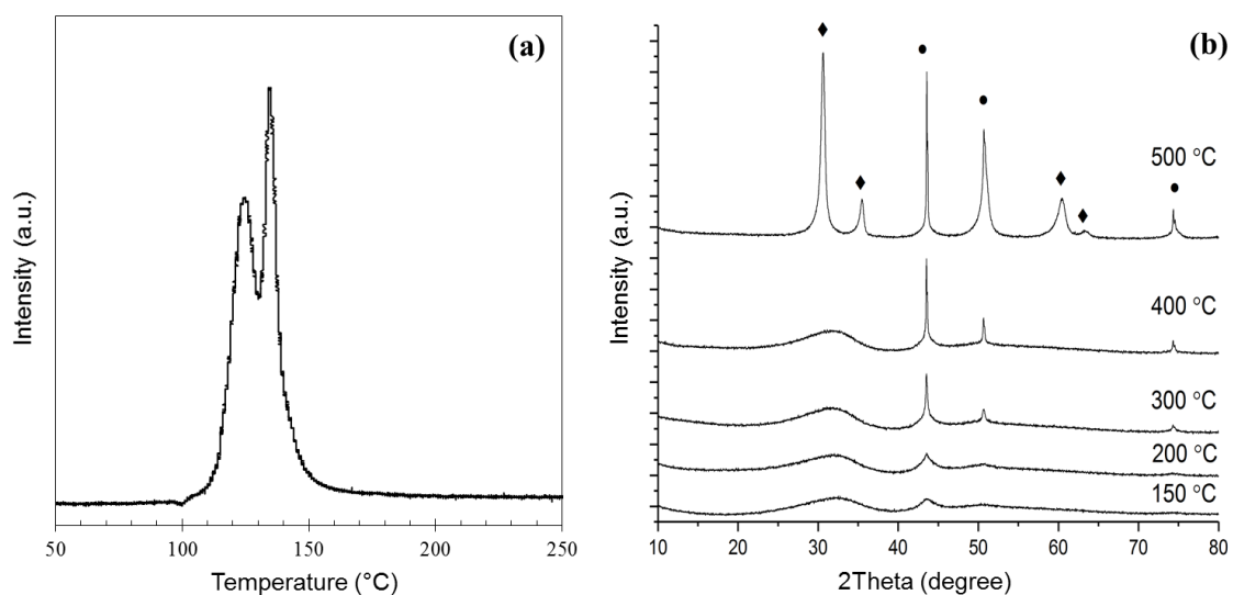
Fig. 9. Temperature programmed reduction of the calcined 30 mol% \text{Cu-ZrO}_2 catalyst with 5% \text{H}_2/\text{Ar} at a ramp rate of 1\text{ }^\circ\text{C}/\text{min} (a). X-ray diffraction patterns of the calcined 30 mol% \text{Cu-ZrO}_2 catalyst after reduction at different temperatures (b).
