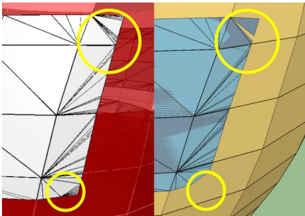
Figure 6. Some slivers (inside the yellow circles) created by the triangulation procedure performed in Dynamo (left) had to be removed when the building was converted to an OpenStudio model (right, visualisation in Sketchup).
