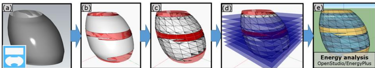
Figure 2. A workflow to create the idealised London City Hall model with bespoke glazing for energy analysis. (a) The input curved target wall and glazing design. (b) The glazing design is applied to the target wall. (c) The wall and its glazing are subdivided and planarised into a set of wall panels. The glazing is mapped to the corresponding wall panel, triangulated, and scaled down by a tiny factor against the panel's boundary. (d) The wall is capped at the bottom and the top to create a closed shape and sliced into multiple stories. In (b), (c), and (d), the building is slightly scaled down for visualisation purposes to avoid rendering otherwise co-planar surfaces. (e) The building model is sent to OpenStudio/EnergyPlus for energy analysis.
