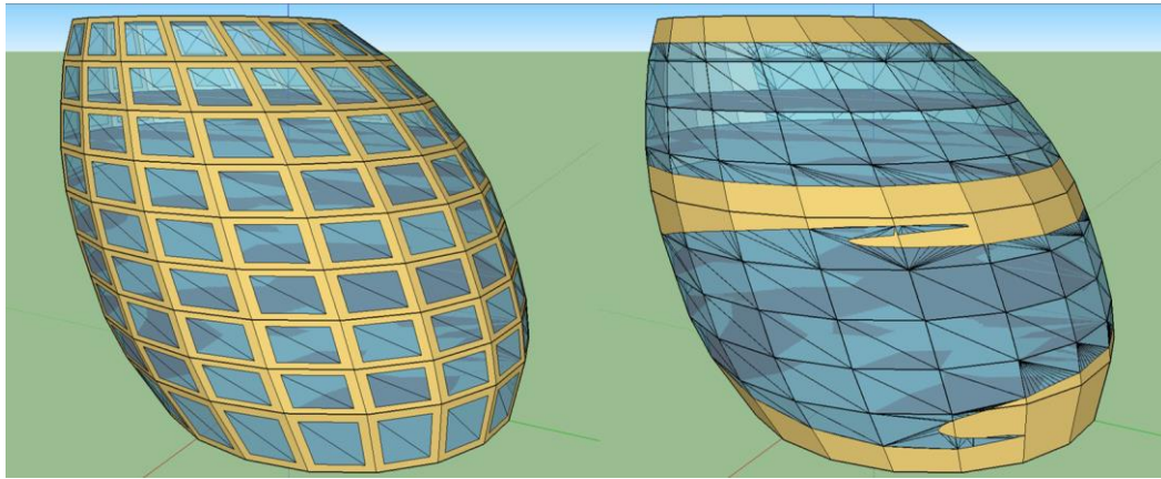
Figure 5. A comparison between the London City Hall model with the glazing defined by (left) window-to-wall ratio and (right) the bespoke design.
