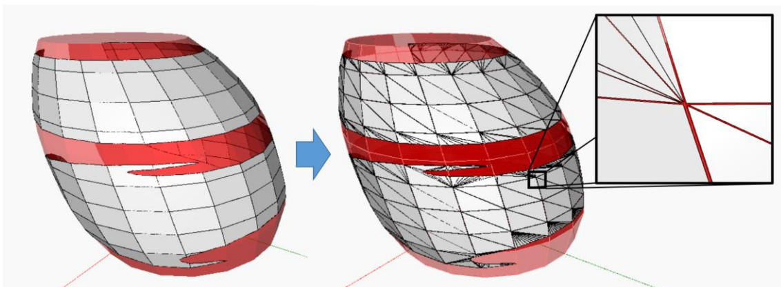
Figure 4. Left: The result of subdividing and planarising the wall and the glazing. Right: The glazing triangulation and scaling down steps result in triangular glazing faces shows the tiny gaps between the faces.
