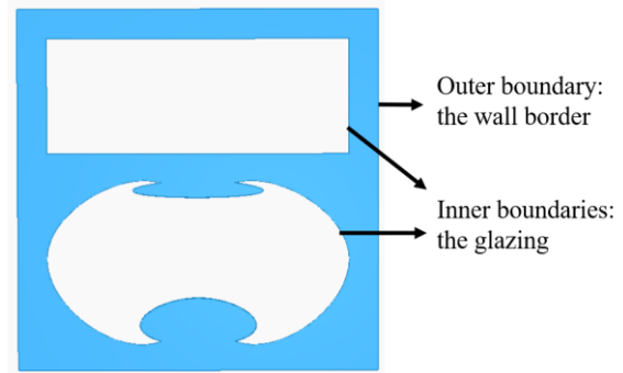
Figure 3. An example of the user-created glazing design with two inner boundaries. The upper inner boundary consists of only straight edges, whereas the lower inner boundary consists of only curved edges.
