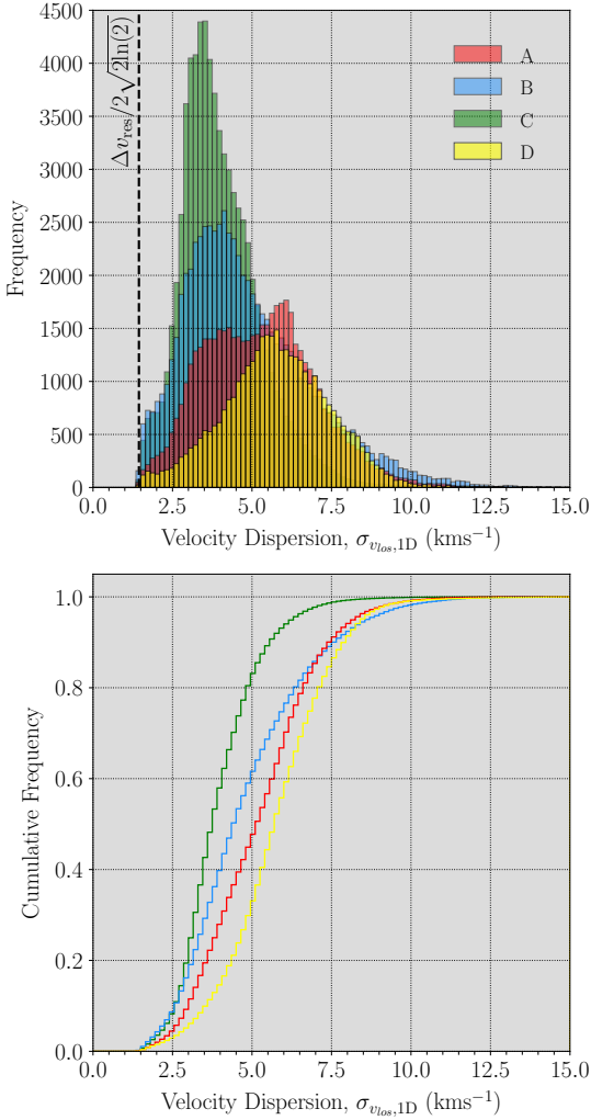
Figure 11. Top: Histograms of the velocity dispersion, \sigma_{v_{los,1D}} , for the main ACORNS trees (coloured histograms; see Figure 5). The vertical line is located at \Delta v_{\text{res}}/2 \sqrt{2 \ln(2)} , where \Delta v_{\text{res}} = 3.4 \text{ km s}^{-1} (the spectral resolution). Bottom: Cumulative histograms of the velocity dispersions for the trees.
