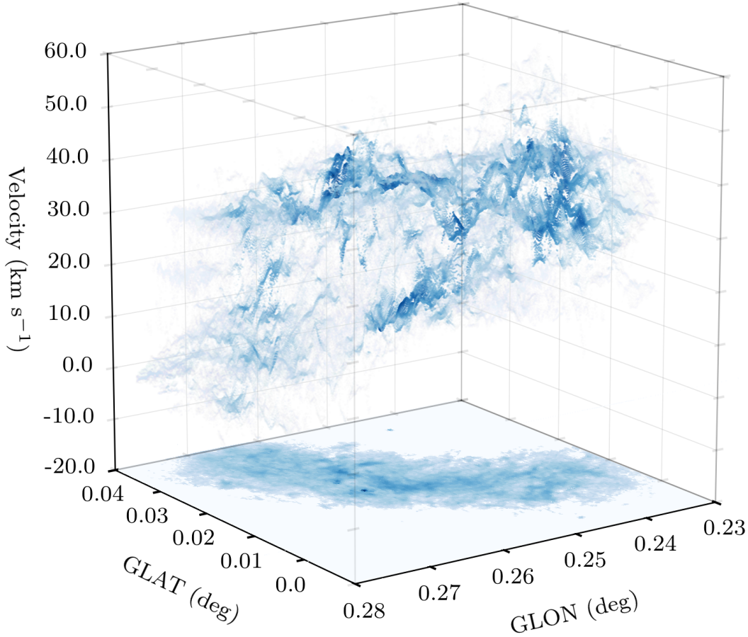
Figure 2. A PPV image of G0.253+0.016. Each data point denotes the location and centroid velocity of a Gaussian component identified in HNC0 emission in the ALMA data and extracted using SCOUSEPY . The colour of each data point (from light to dark) is proportional to the peak intensity of the corresponding spectral component. Note that only the data between -20.0 \text{ km s}^{-1} and 60.0 \text{ km s}^{-1} are shown. Emission outside of this velocity range, although spatially coincident with G0.253+0.016 may not be associated with the cloud itself. The full extent of the data can be seen in Figure 3. At the base of the plot, we plot the 3 mm dust continuum emission first presented in Rathborne et al. (2015). This figure highlights the kinematic complexity of G0.253+0.016.
