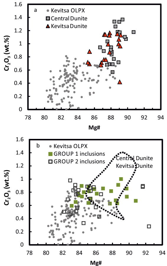
Figure 9. Cr 2 O 3 (wt.%) vs. Mg# plot for clinopyroxene from the Central Dunite, Kevitsa Dunite, and Group 1 and Group 2 inclusions. Clinopyroxene compositions of Kevitsa olivine pyroxenites (OLPX) from unpublished data by the first author.
