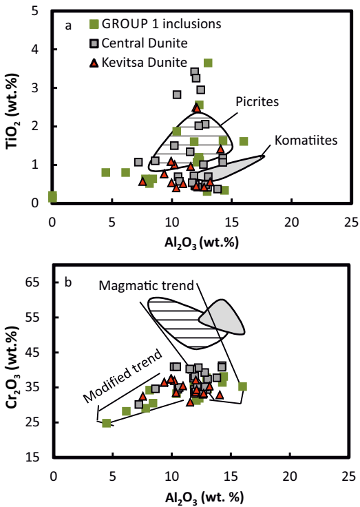
Figure 8. a) TiO 2 vs. Al 2 O 3 and b) Cr 2 O 3 vs. Al 2 O 3 (b) plot for chromite from the Central Dunite, Kevitsa Dunite, and Group 1 inclusions. The magmatic chromite trend after Bliss and Maclean (1975) and the modified trend after Wang et al. (2005). Chromite compositions in picritic and komatiitic volcanic rocks (Savukoski Group) from Hanski and Kamenetsky (2013).
