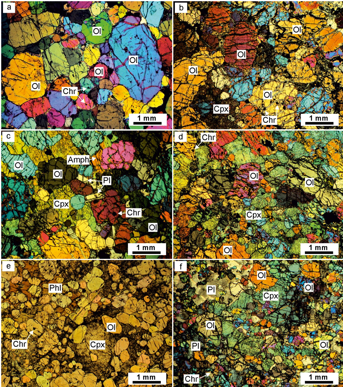
Figure 4. Photomicrographs of dunitic cumulates. a) Dunitic adcumulate (Central Dunite); b) Moderately altered dunitic adcumulate (Kevitsa Dunite); c) Wehrlite (Central Dunite); d) Wehrlite (Kevitsa Dunite). Single clinopyroxene oikocryst fills the entire picture; e) Wehrlite (feldspathic but all plagioclase altered to chlorite, not shown). Note the reduced olivine grain size (Central Dunite); f) Fine-grained feldspathic wehrlite (Kevitsa Dunite). Figures a-d and f taken with crossed polars and e with parallel polars. Ol = olivine, Cpx = clinopyroxene, Chr = chromite, Pl = plagioclase, Phl = phlogopite, Amph = amphibole.
