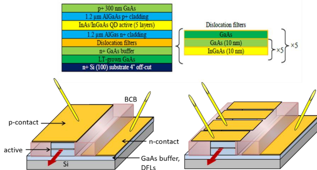
Fig. 1. (a) Schema of epitaxial growth structure including details of defect filters and (b) Ridge-waveguide on Si substrate laser (left) and segmented contact test structure (right).
