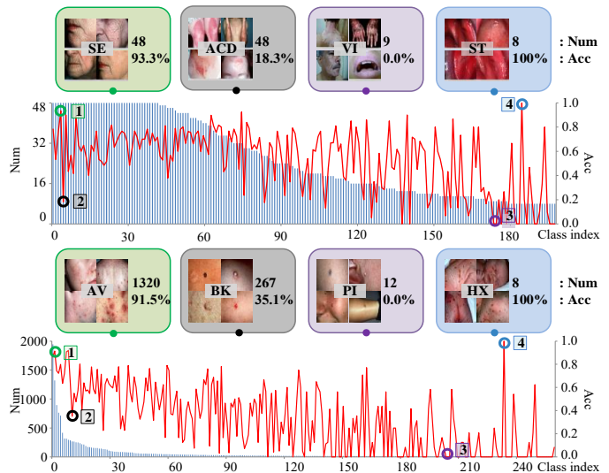
Fig. 1: Visualization of the class distribution in the SD-198 [4] (top) and SD-260 (bottom) datasets. The blue bars denote the number of training samples (Num) for each class, while the red line denotes the classification accuracy (Acc) of the raw ResNet50 [6] on the testing set. Each colored box visualizes a specific skin disease, e.g. , solar elastosis (SE), allergic contact dermatitis (ACD). The numbers in the boxes report the number of samples and the recognition accuracy, respectively.
