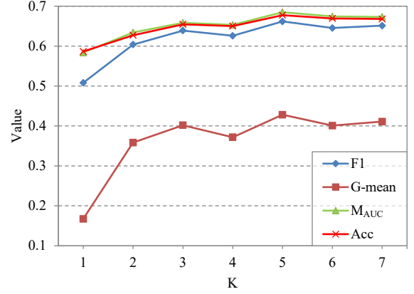
Fig. 3: Classification performance of the proposed SPBL method with different total number of paces ( K ). Here, “value” indicates the results of F1 , G -mean, M_{\text{AUC}} and Acc (accuracy) on the SD-198 dataset. Accordingly, we set K = 5 in the rest of the experiments, i.e. , we conduct 5 paces for each experiment.
