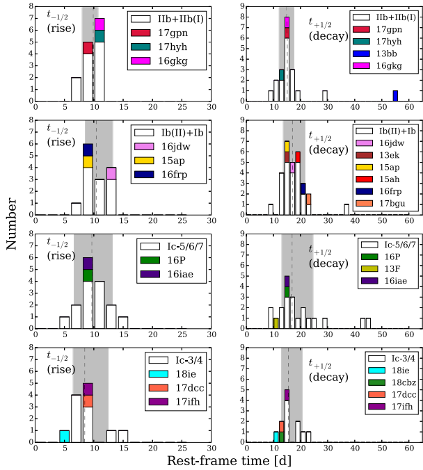
Figure 10. Distributions of t_{-1/2} (left) and t_{+1/2} (right) for the various SN subtypes. SN I Ib(I) 2013bb is a clear outlier with t_{+1/2} \sim 56 d. The dashed line and grey regions are as in Fig. 9.
