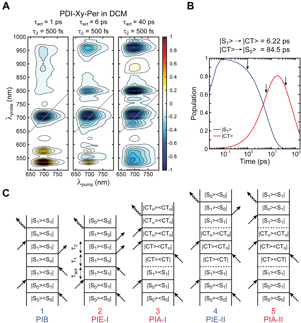
Figure 2. (A) t-2DES spectra of PDI-Xy-Per in DCM as a function of the actinic pump delay ( \tau_{act} ). The spectra are normalized to the maximum absolute change in absorption at each ( \tau_{act} , \tau_2 ). (B) Population evolution of different states obtained from the evolution-associated spectral analysis of conventional 2DES data on PDI-Xy-Per in DCM. The black arrows indicate the actinic delays used for measurement of t-2DES spectra. (C) Feynman diagrams corresponding to representative pathways resulting different types of t-2DES spectral features. The dotted horizontal lines indicate population transfer during the time period between two light-matter interactions.
