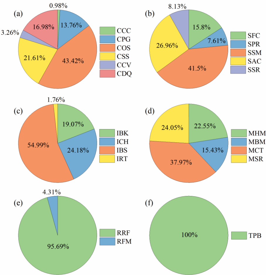
Fig. 5 Contribution of each emitting point to the TEIS of each process: (a) coking, (b) sintering, (c) ironmaking, (d) steelmaking, (e) steel rolling, and (f) thermal power.
