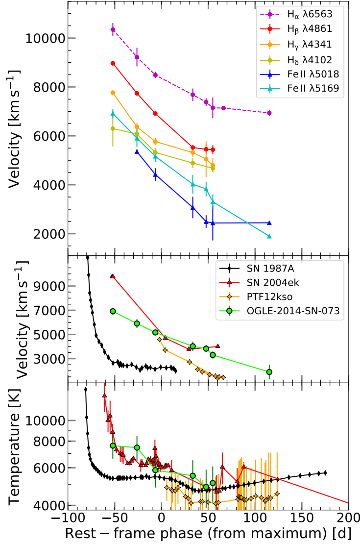
Supplementary Figure 3: Line velocity and temperature evolution of OGLE14-073
