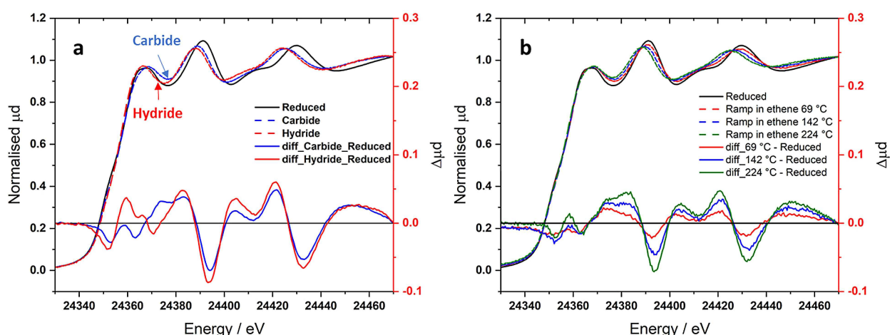
Figure 3. (a) Normalised Pd K edge XANES spectra of Pd 0 , Pd hydride and Pd carbide. The difference spectra ( -\text{Pd}^0 reference) of Pd carbide and Pd hydride are also shown. (b) Normalised Pd K edge XANES spectra during time-resolved ethene decomposition (temperatures of 69 °C, 142 °C, 224 °C) alongside associated difference spectra.
