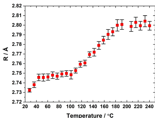
Figure 2. In situ measurements of the average lattice expansion of the Pd nanoparticles exposed to ethene as a function of temperature of the sample.
