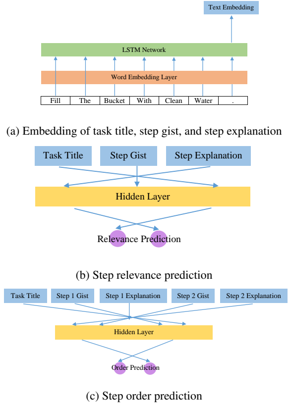
Figure 1: Model architecture
