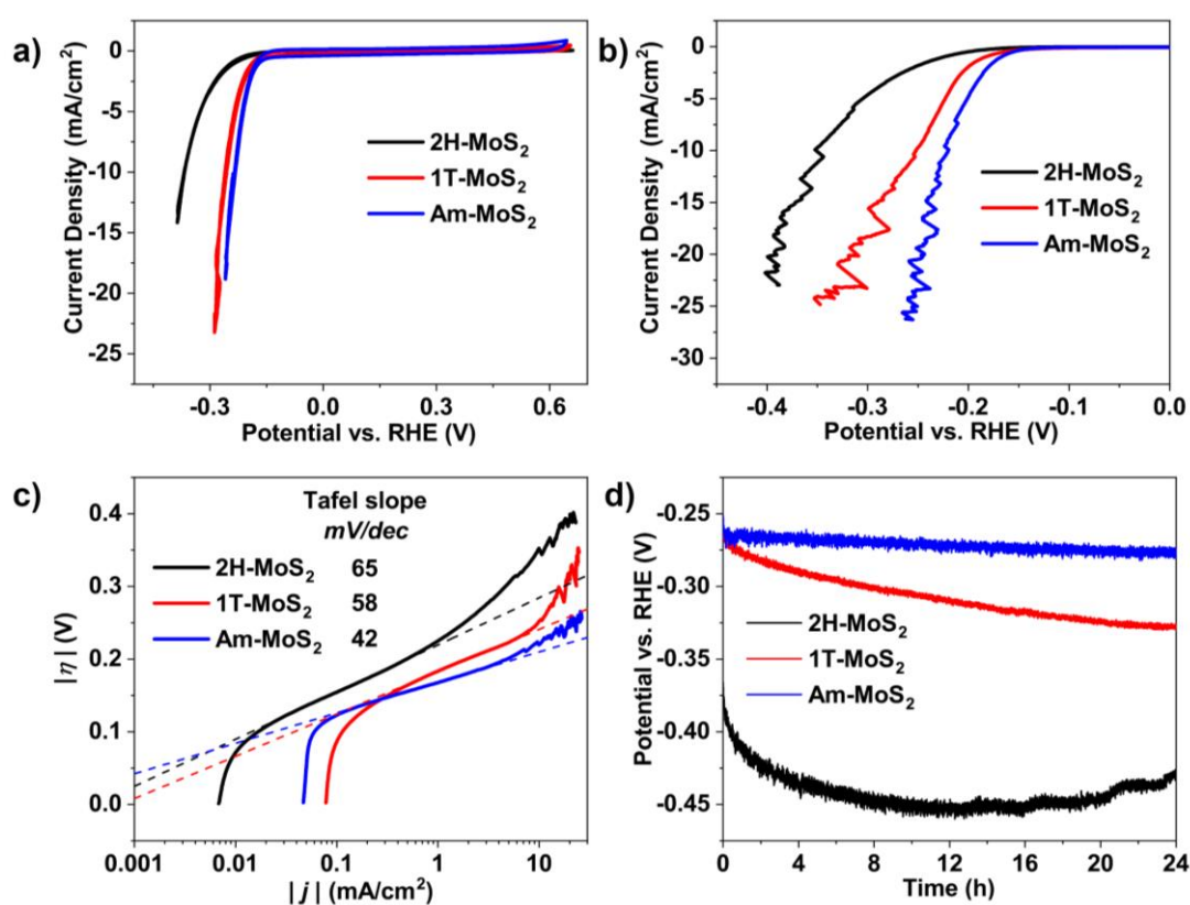
Figure 1. Cyclic voltammetry (CV, a) and linear sweep voltammetry (LSV, b) curves of 2H-, 1T- and Am-MoS 2 films corrected by uncompensated resistance with scan rates of 50 mV/s for CV and 5 mV/s for LSV; c) Tafel slopes obtained from LSV curves in (b); d) chronopotentiometric responses ( V-t ) recorded at a constant current density of 3 mA/cm 2 . Electrolyte: 0.1 M H 2 SO 4 .
