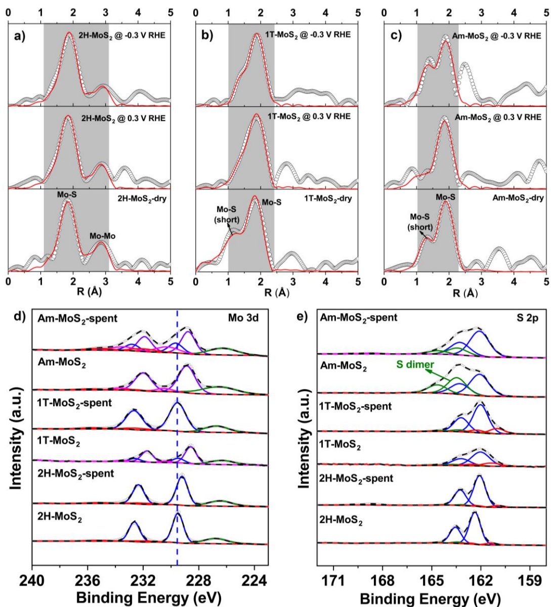
Figure 3. a-c) Mo K-edge Fourier transform EXAFS ( k^2 -weighted) of 2H- (a), 1T- (b) and Am- (c) MoS 2 under operando electrochemical conditions, grey region represents R-range for fitting; d, e) X-ray photoemission spectra of Mo 3d (d) and S 2p (e) before and after (-spent) operando XAS measurements.
