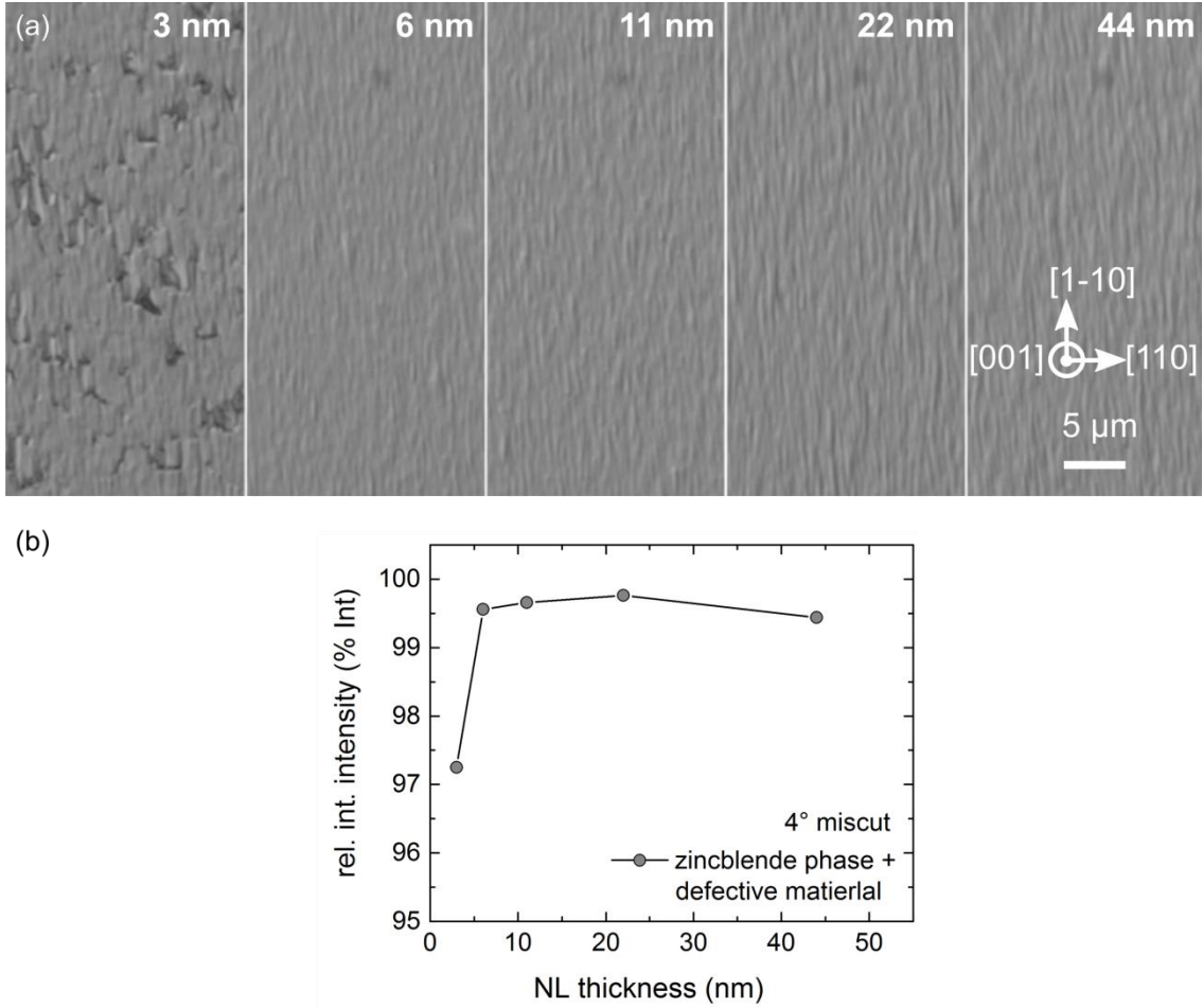
Figure 10 (a) Normarski images of the GaN epilayers grown on NLs with different thicknesses. (b) The sum of the relative integrated intensity of zincblende phase and defective material peaks in the zb-GaN epilayers grown on NLs with different thicknesses, as determined by XRD.
