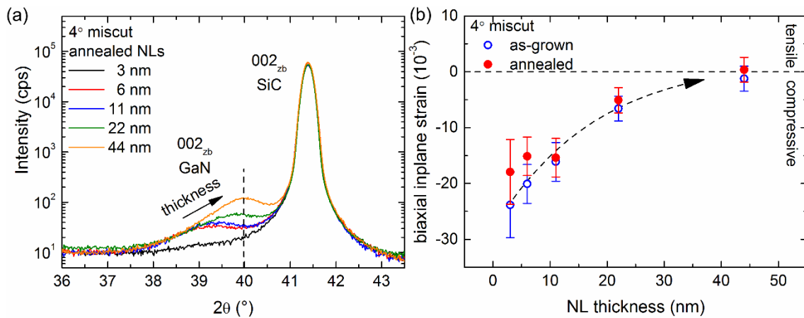
Figure 8 (a) XRD \omega 2\theta -scans of the 002 zb-GaN and SiC reflections for the annealed NLs grown on the 4° miscut substrate. The dotted line marks the position of relaxed zb-GaN. (b) The dashed line provides a guide-to-the-eye showing the change in bi-axial in-plane strain
