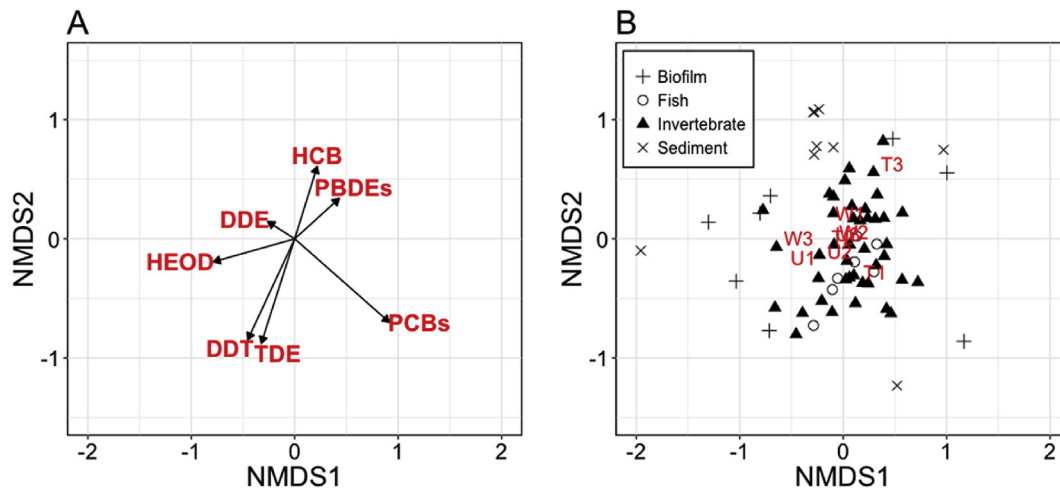
Fig. 2. Concentration and composition of POPs across sites and sample types (sediments, biofilms, invertebrates and fish). (A) NMDS of POP congeners and chemicals across sites (n = 9) and catchments (n = 3). (B) Variation in POP composition between sample types.
