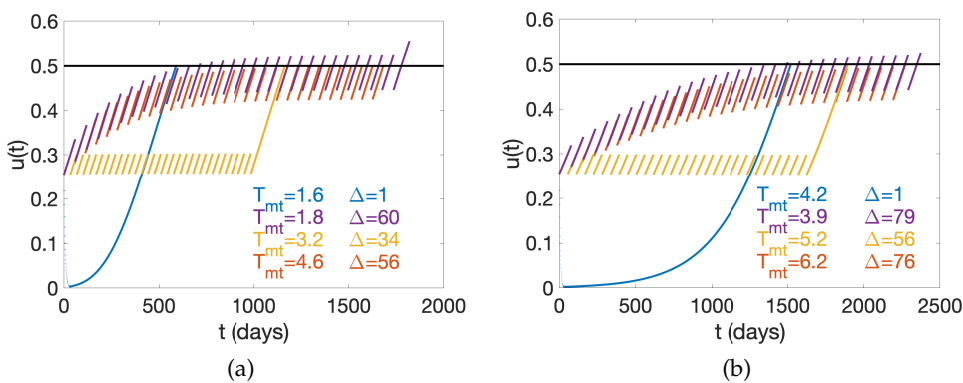
Figure 9. (a) Gompertz growth, with \rho = 0.003756 \text{ day}^{-1} , S = 0.85 , u_1 = 0.3 and u_* = 0.5 . (b) Logistic growth, with \rho = 0.004 \text{ day}^{-1} , S = 0.85 , u_1 = 0.3 and u_* = 0.5 . Units for T_{mt} and \Delta are years and days, respectively. Blue curve corresponds to the standard protocol, purple curve corresponds to the optimal protocol for a wrong u_* , yellow curve corresponds to sub-optimal protocol and red curve corresponds to optimal protocol. Black horizontal line represents u_* .
