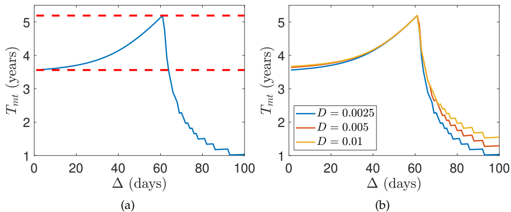
Figure 7. (a) Prediction of the time to the malignant transformation given by the Fisher-Kolmogorov equation in one dimension for different spacing between doses for D = 0.0025 \text{ mm}^2/\text{day} . (b) Prediction of the time to malignant transformation given by the Fisher-Kolmogorov equation in one dimension for different spacing between doses and different values of the diffusion coefficient. For all the simulations, the values of the parameters used were S = 0.85 , u_1 = 0.3 , u_* = 0.5 , \rho = 0.005 \text{ day}^{-1} and \sigma = 10 \text{ mm}^2 . Upper and lower red dashed lines in the figures corresponds to T_{mt}(\Delta_{Opt}) and T(1) , respectively, (see Eq. (2.11))
