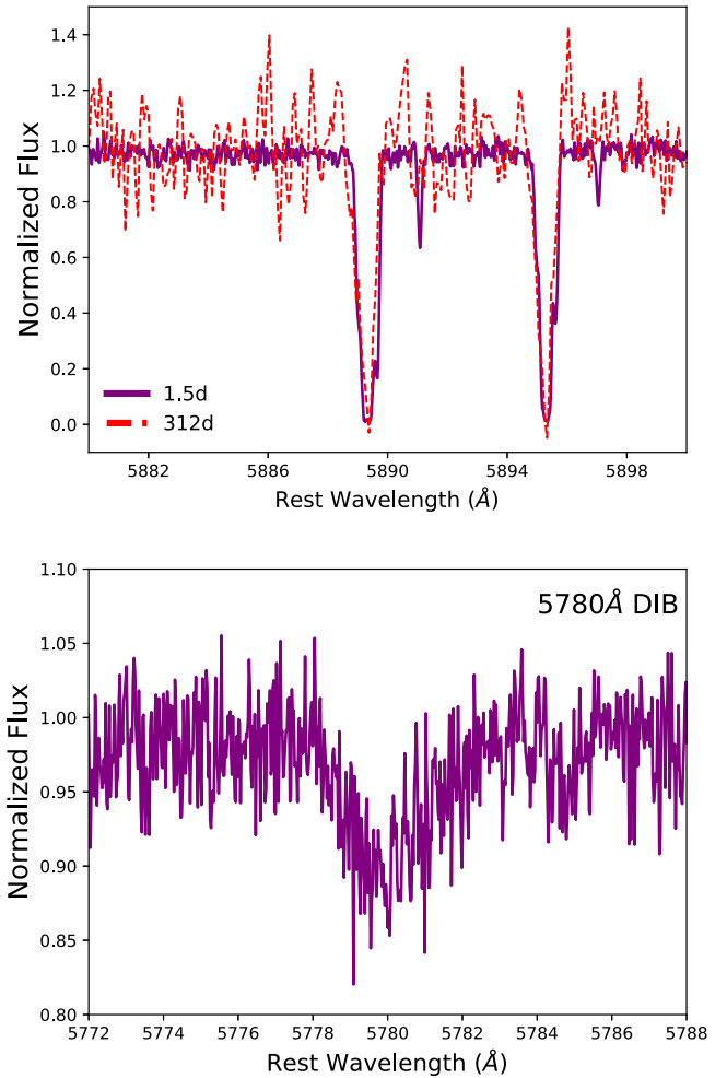
Figure 2. Keck HIRES spectra (purple) from day 1.5 showing the region around the Na I D lines (top) and the \lambda 5780 \text{ \AA} DIB feature (bottom). The red Na I D spectra is from Magellan/MIKE echelle spectra on day 312.
