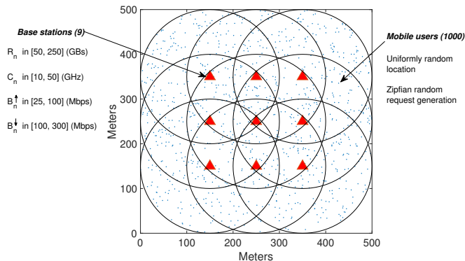
Fig. 3: Evaluation setup.
