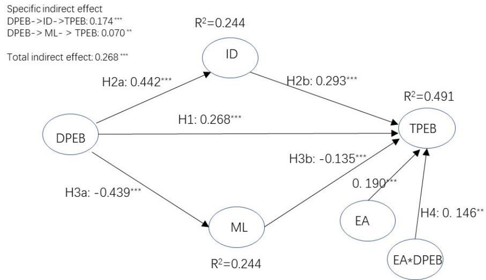
Fig. 1 PLS-SEM results
